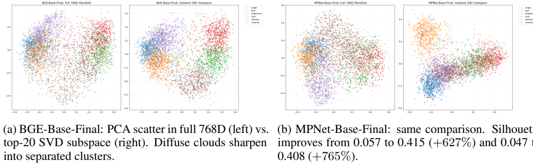
Figure 4: 768D vs. top-20 SVD subspace (Finding 3). Projecting into the 20-dimensional signal subspace reveals the cluster structure hidden by noise dimensions in the full embedding space.
