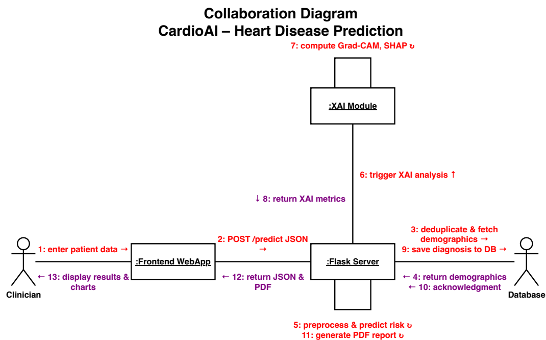
Figure 2.12: UML Collaboration Diagram highlighting the structural communication links between components.
