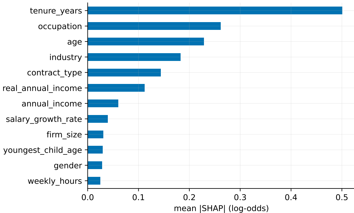
SHAP global feature importance
