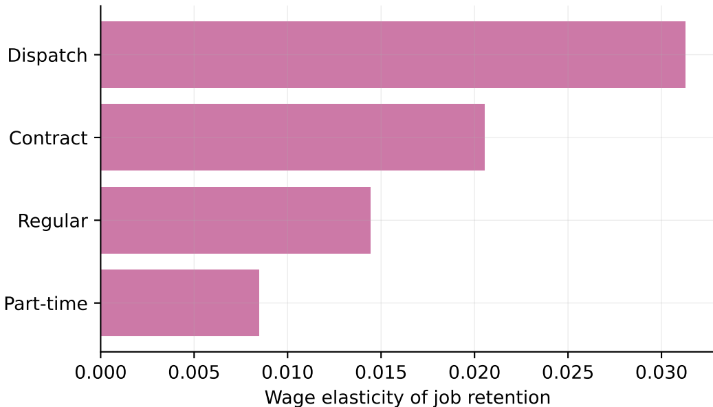
Extensive-margin labour-supply elasticity by contract type
