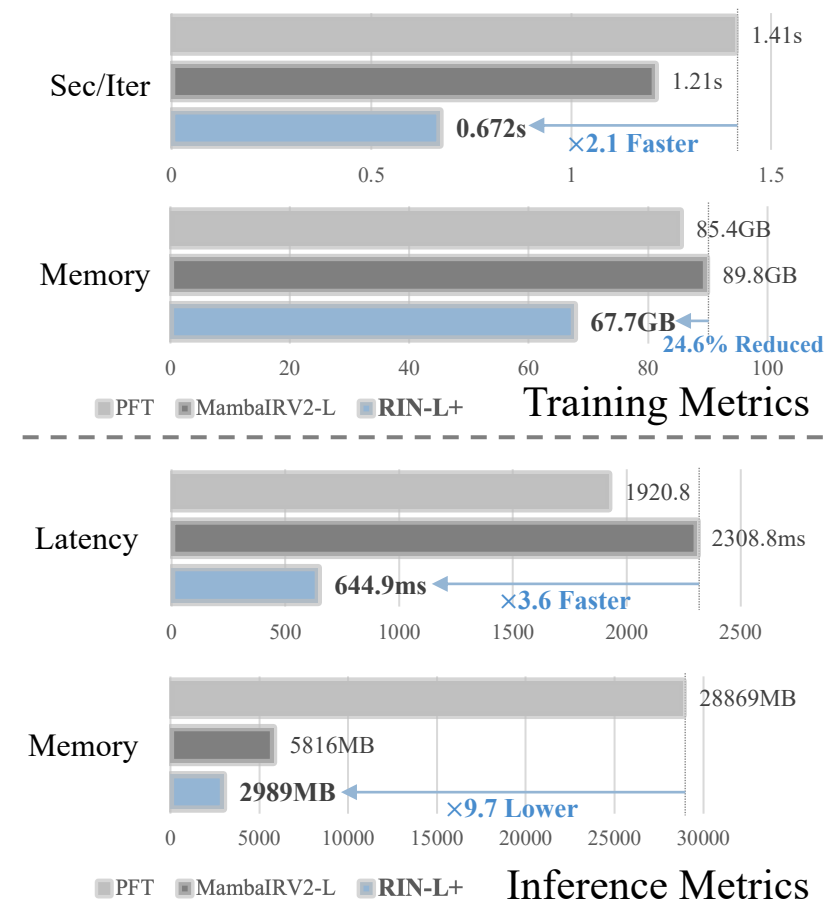
Efficient Training/Inference
