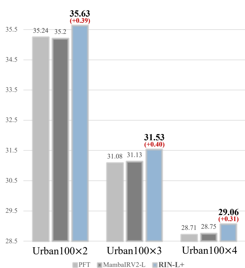
Improved Performance
