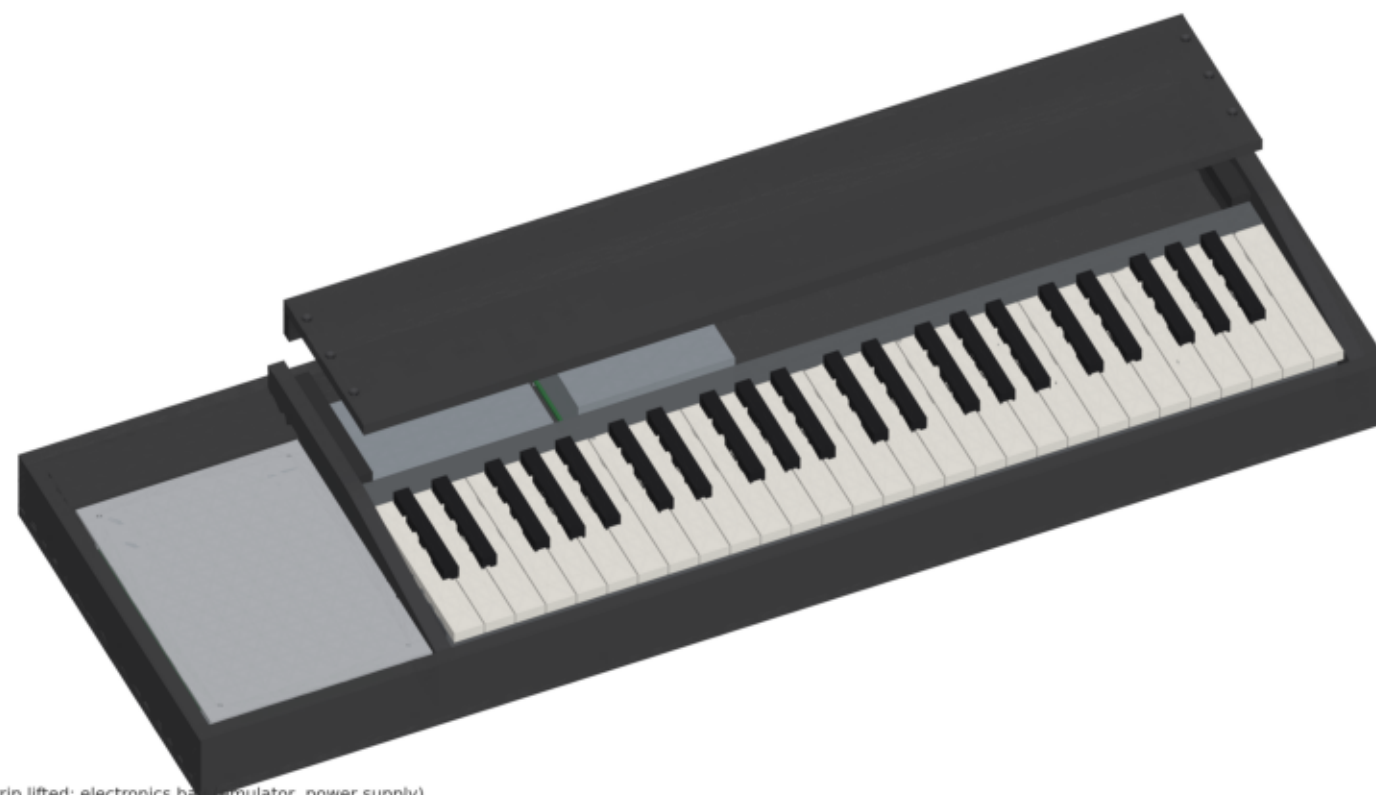
strip lifted: electronics bay (emulator, power supply)
