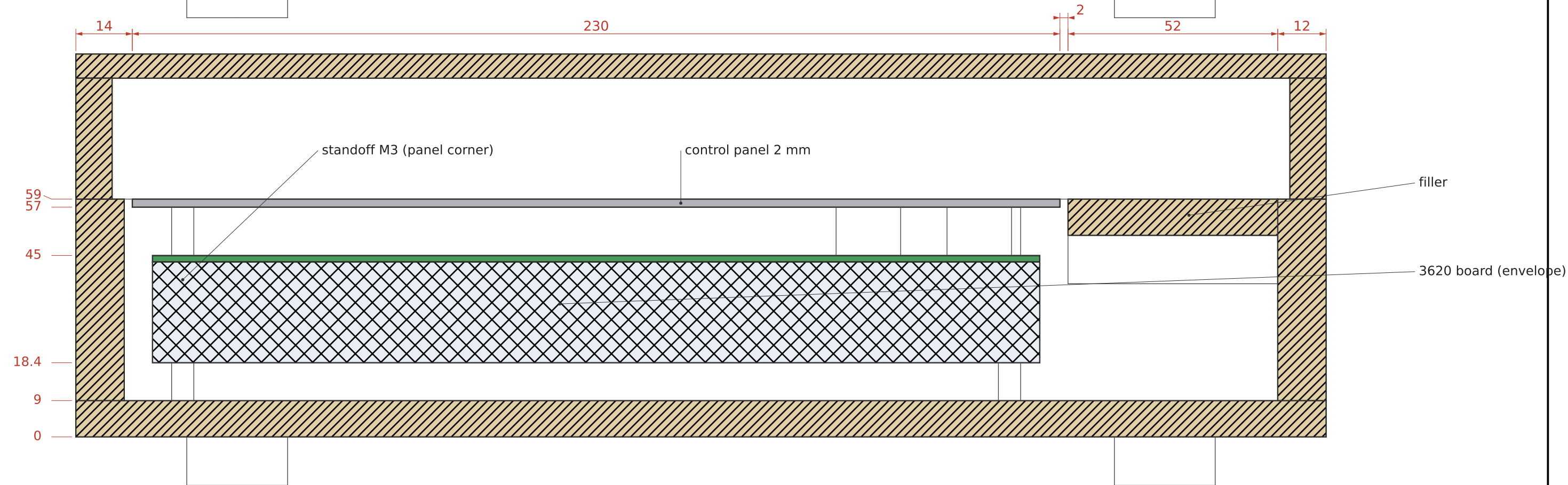
Section B-B at x = 100 (control panel)
