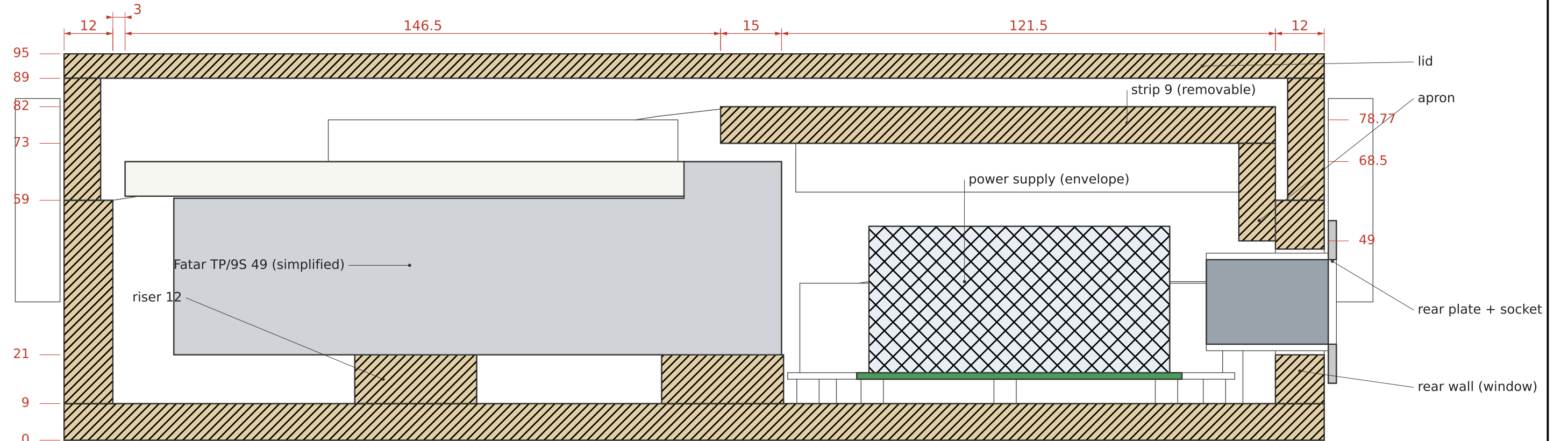
Section B-B at x = 100 (control panel)
