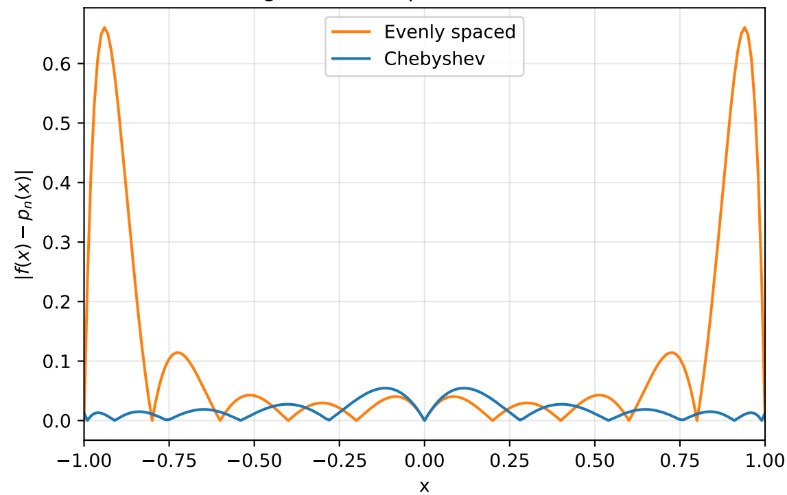
Degree 10: sampled absolute error
