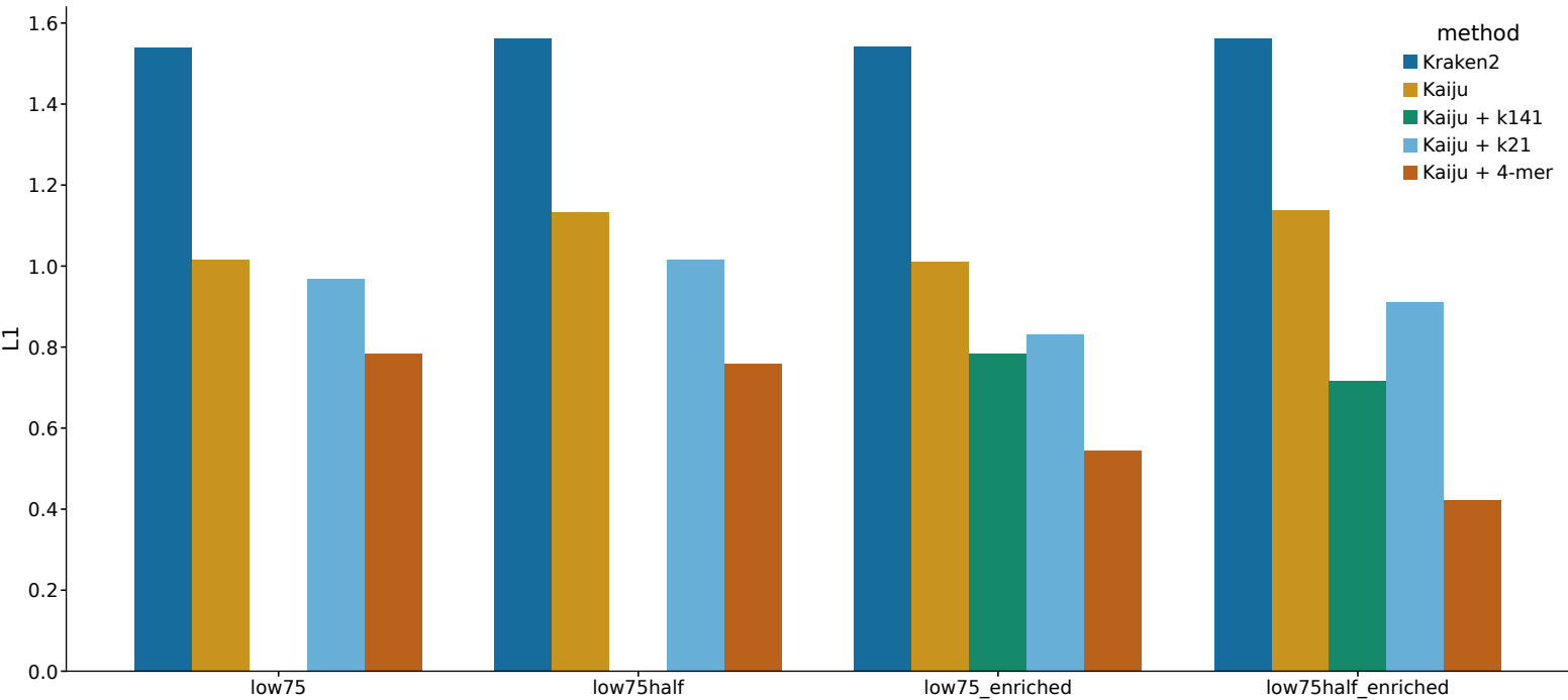
Genus L1 on reads
