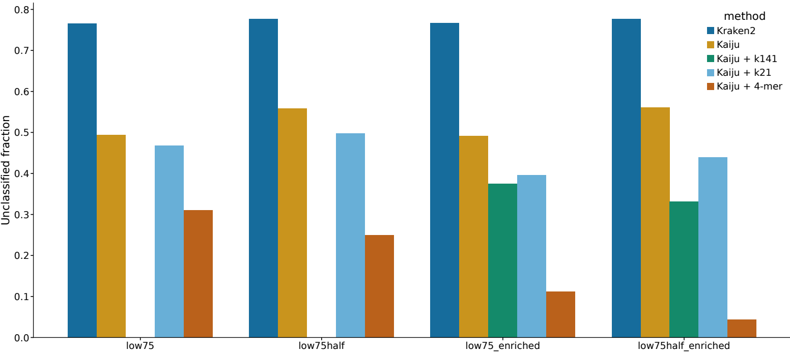
Unclassified read fraction at genus
