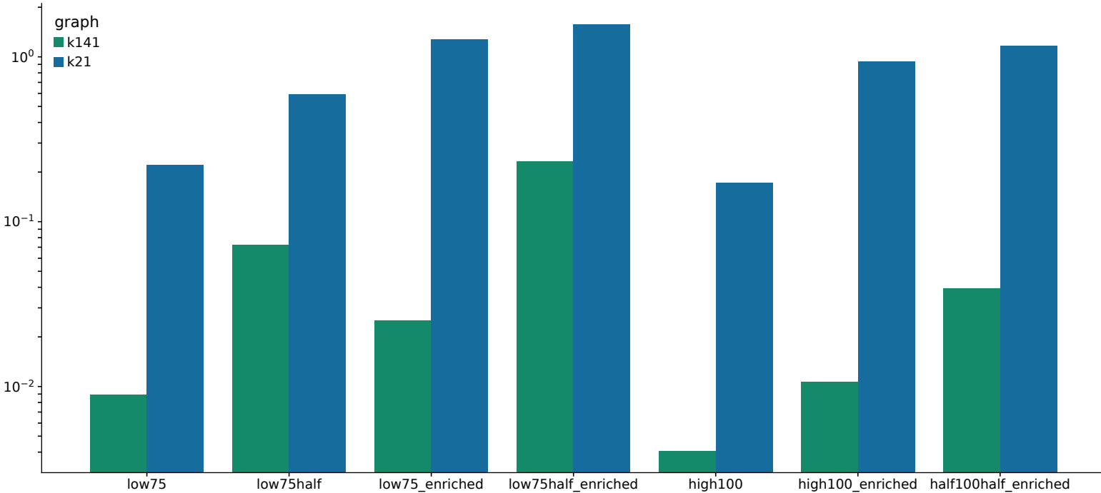
MEGAHIT graph density
