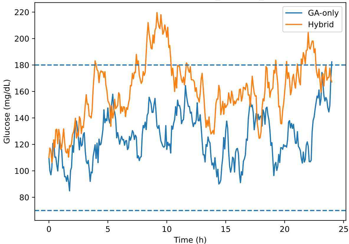
Glucose trajectory G(t) — S4_exercise_lowcarb
