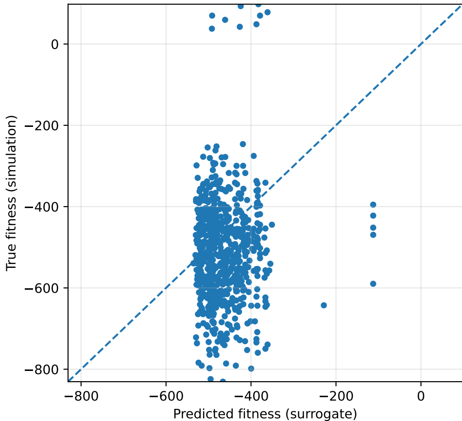
GA+Surrogate accuracy (S4)
