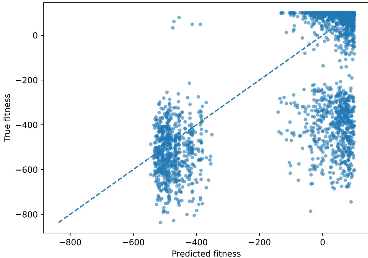
GA+Surrogate: predicted vs true fitness
