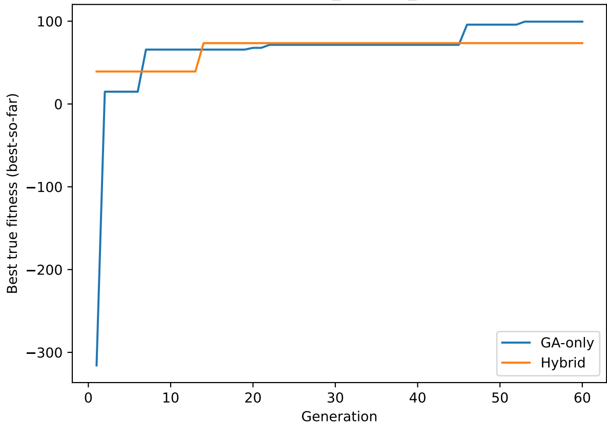
Convergence (S4_exercise_lowcarb)
