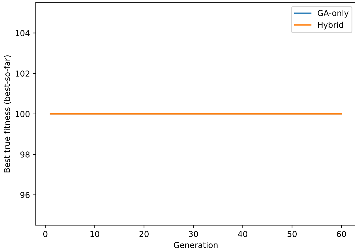
Convergence (S3_stress_highcarb)
