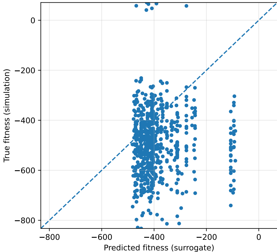
Hybrid surrogate accuracy (S4)
