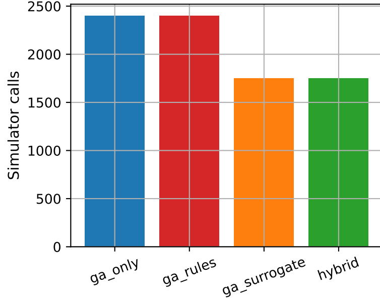
(c) Average Simulation Cost
