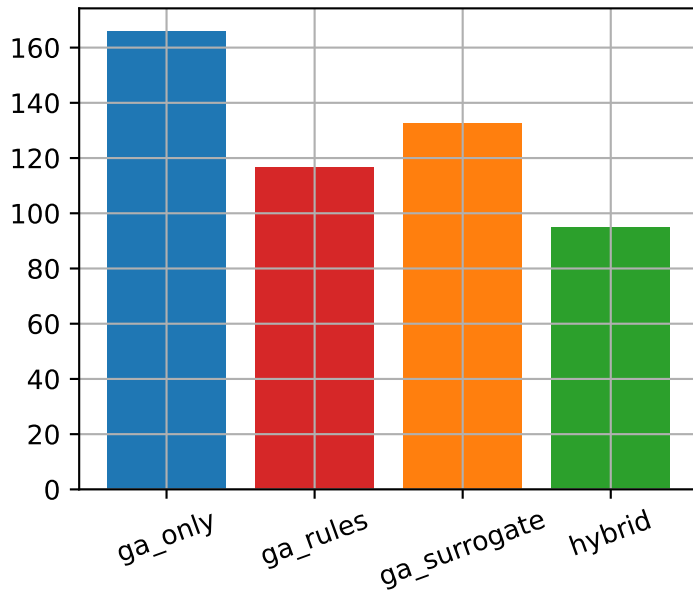
(b) Average Convergence Regret
