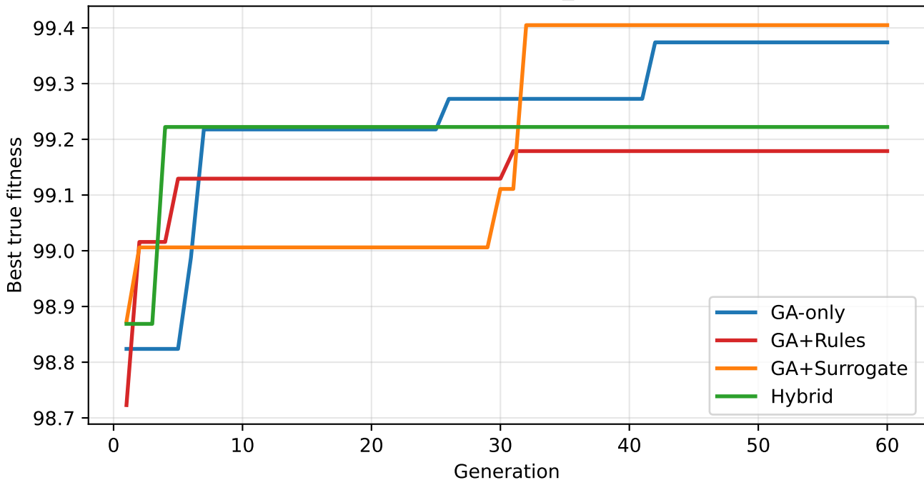
Convergence - S1_normal
