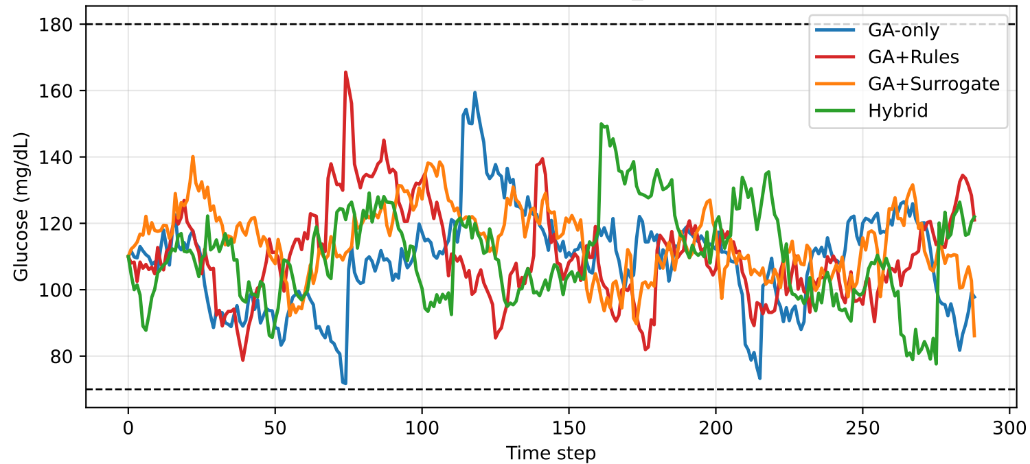
Glucose Trajectories - S2_ramadan
