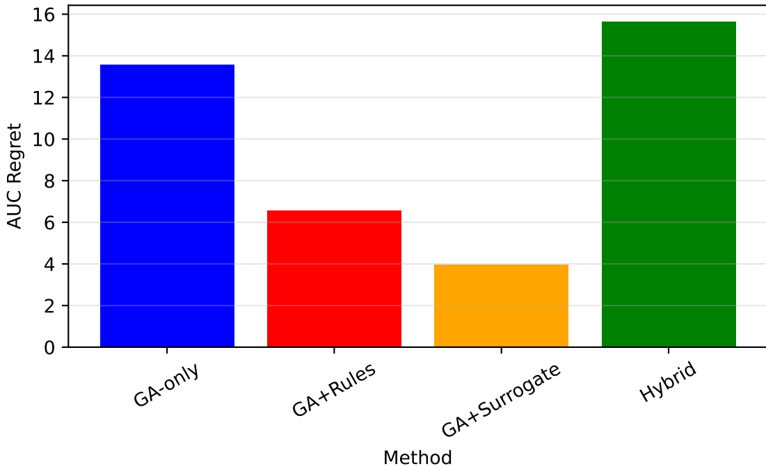
Convergence Regret - S2_ramadan
