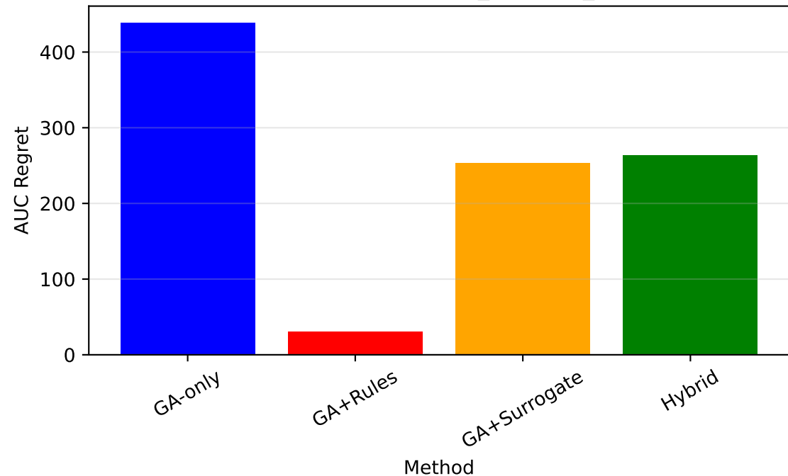
Convergence Regret - S4_exercise_lowcarb
