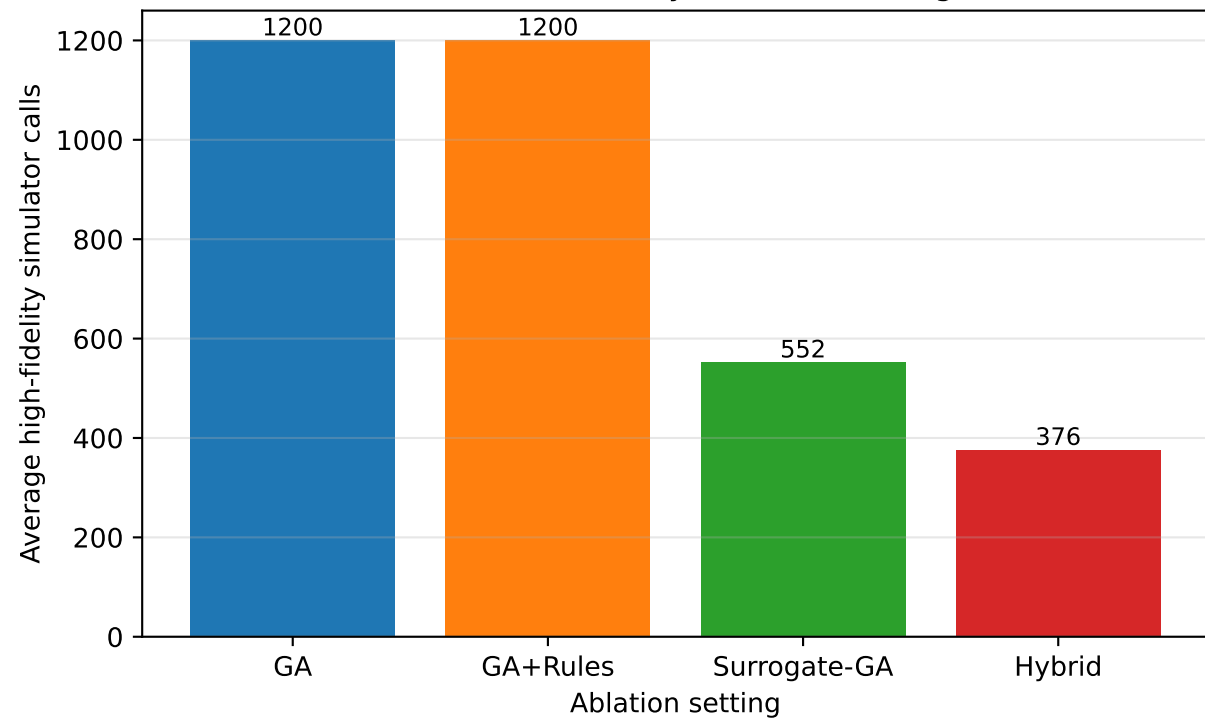
Simulator Calls by Ablation Setting
