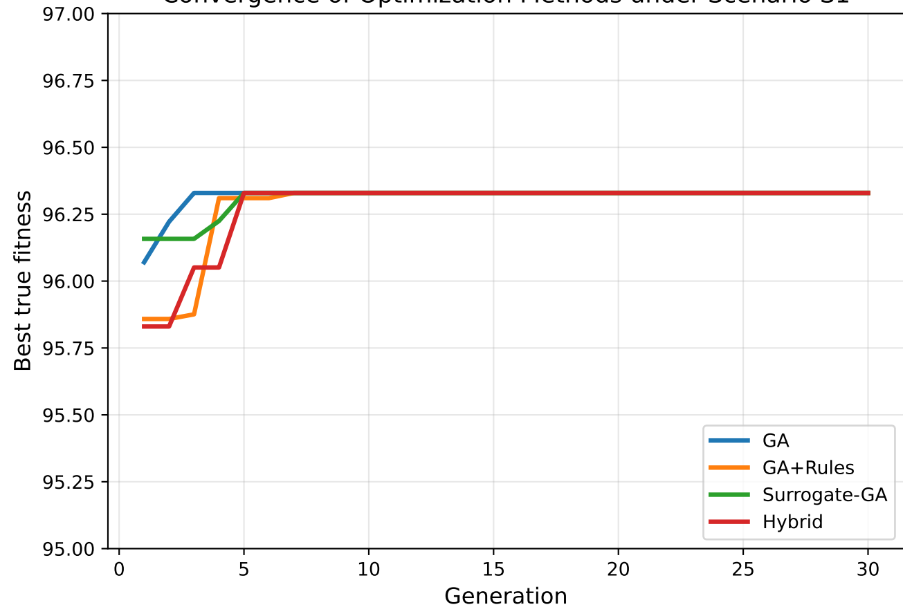
Convergence of Optimization Methods under Scenario S1
