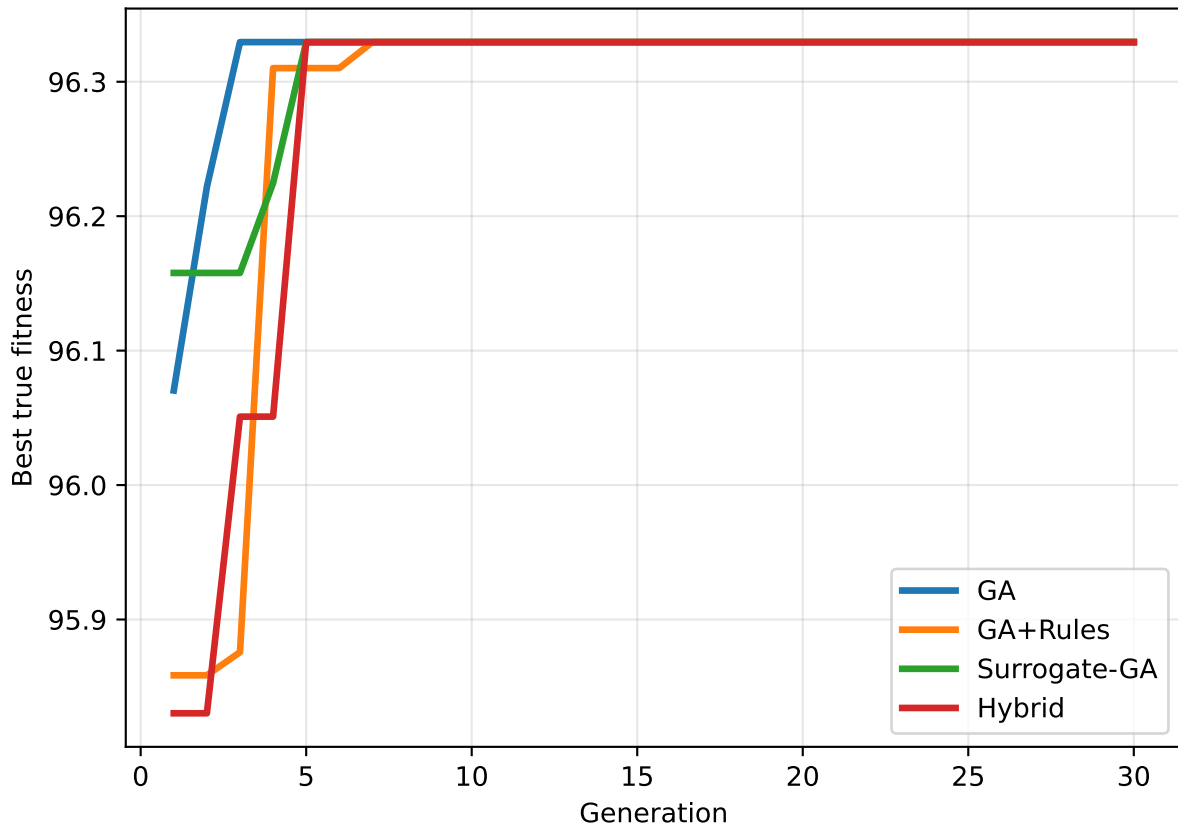
Convergence of Optimization Methods under Scenario S1
