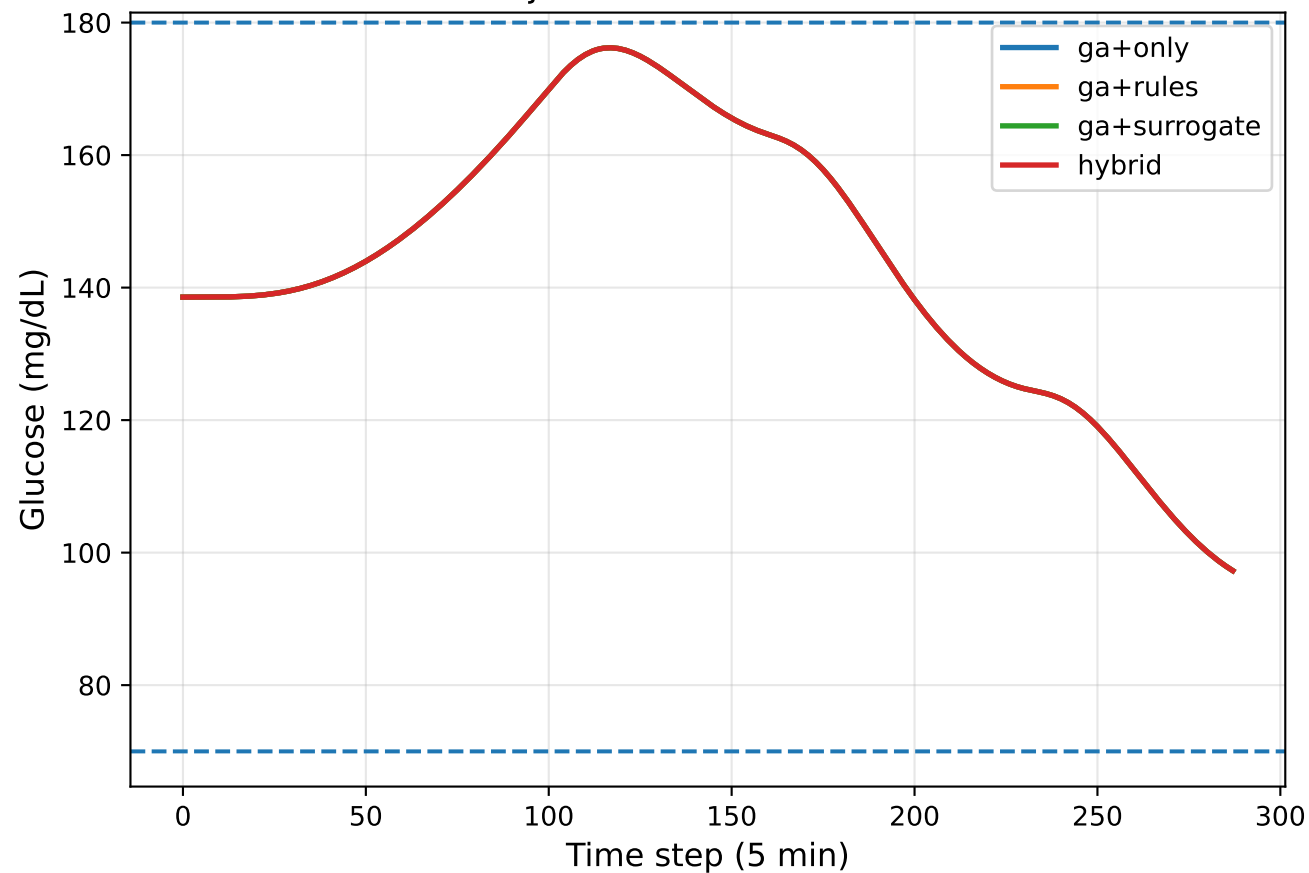
Glucose Trajectories under Normal Scenario
