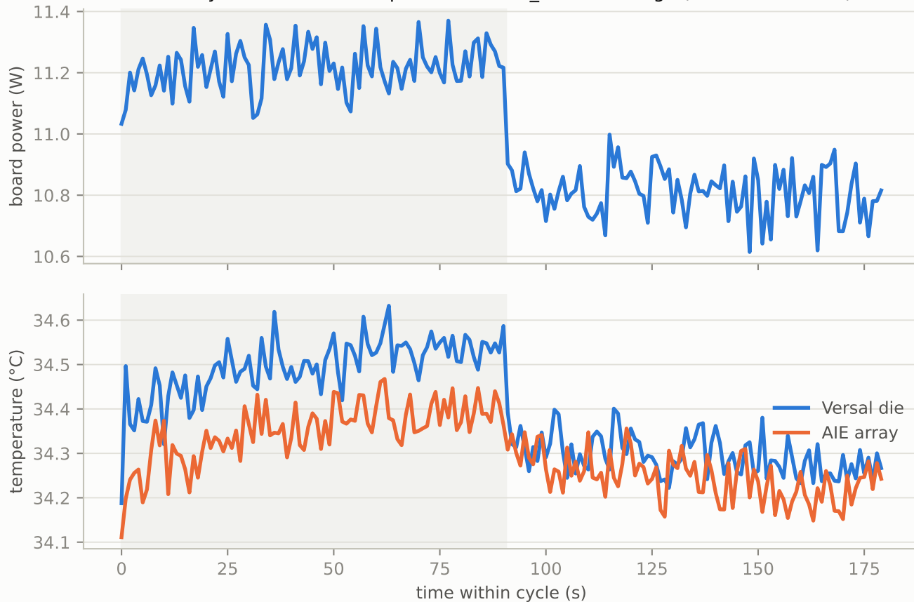
Folded load cycle, mean of 16 repetitions — aie_maskfix image (shaded: load ON)
