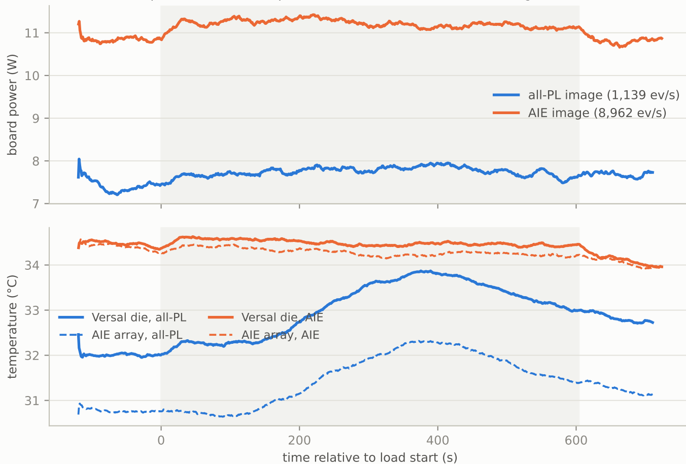
VCK190 board power and die temperature vs time — all-PL vs AIE image (shaded: sustained load)
