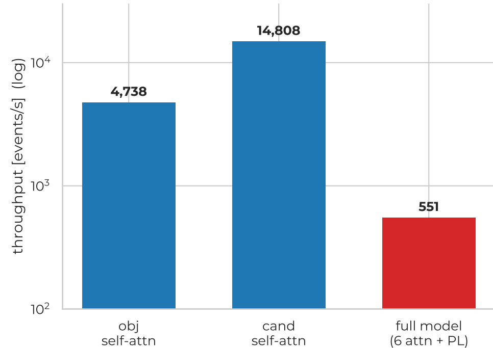
Measured throughput (HW, golden-fed) attention block >> full model
