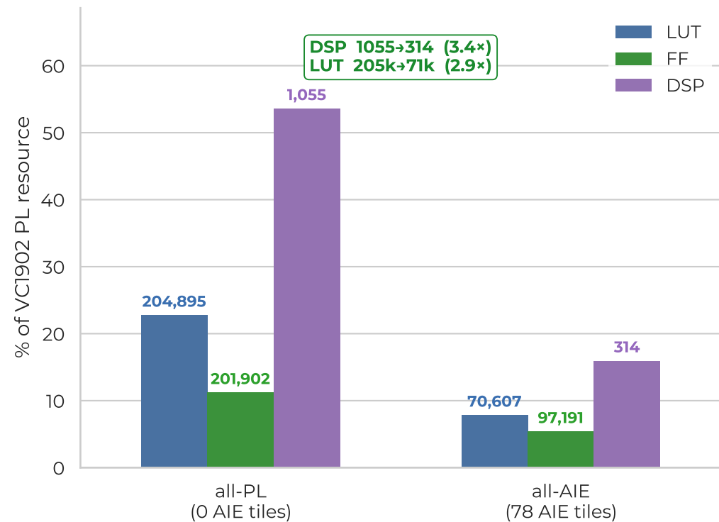
PL fabric: all-PL vs all-AIE (full model, measured)
