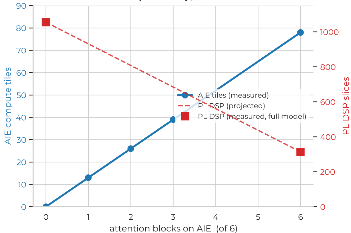
Scale AIE up → tiles up, PL DSP down
