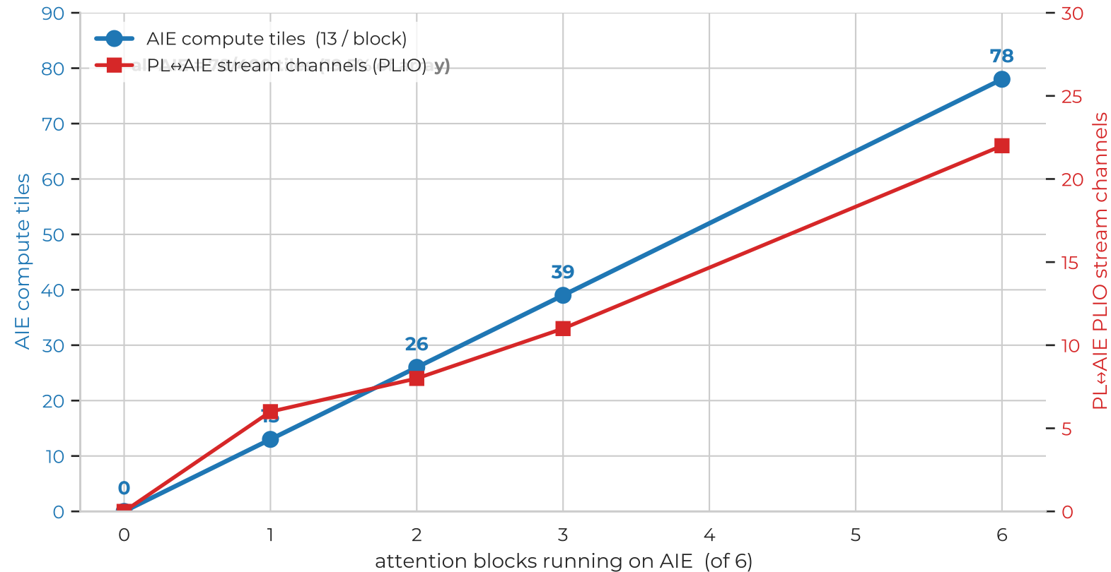
Scaling AIE usage: tile & stream cost is linear in blocks offloaded
