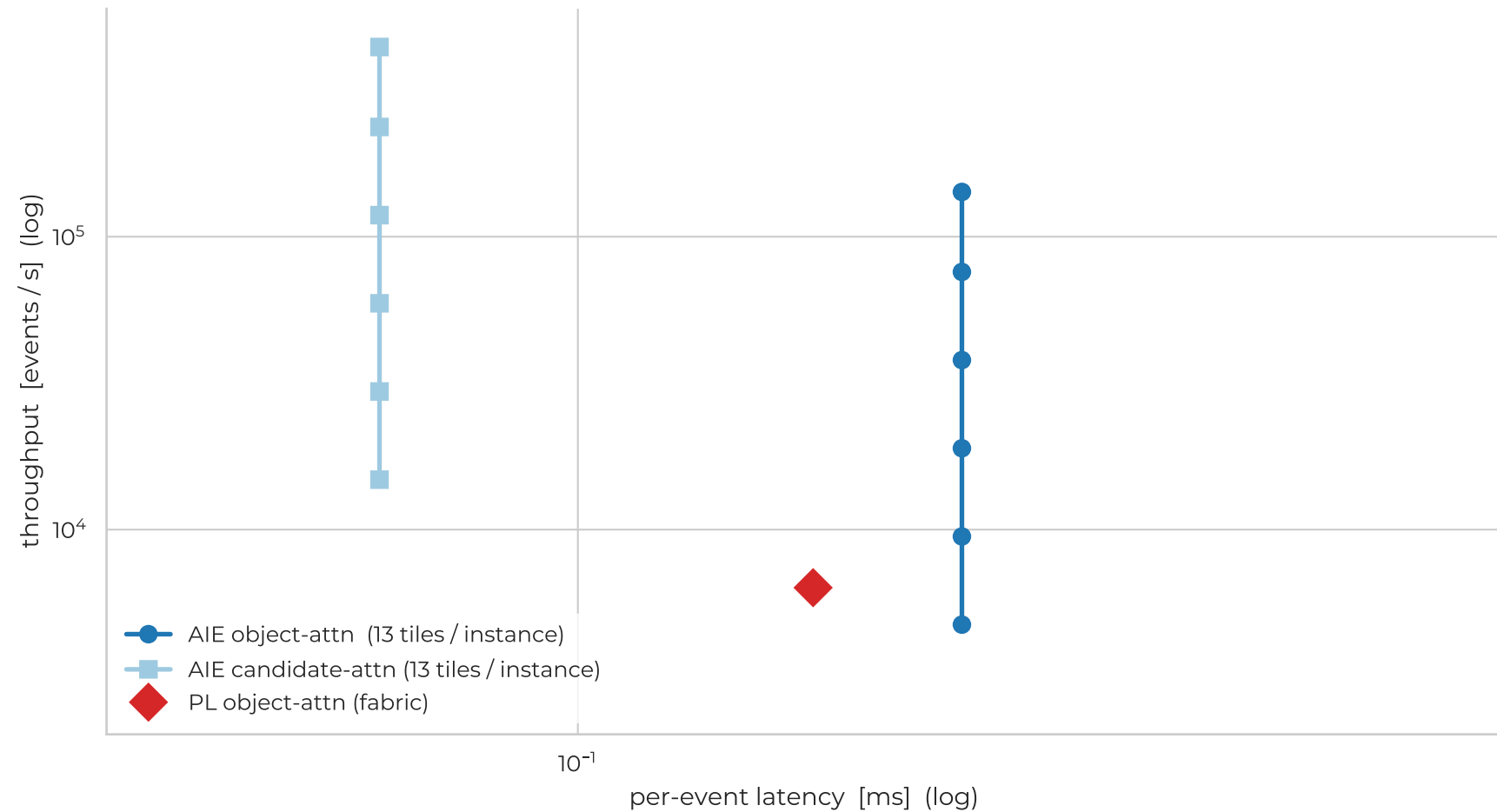
Attention blocks: latency vs throughput (AIE scales with tile count)
