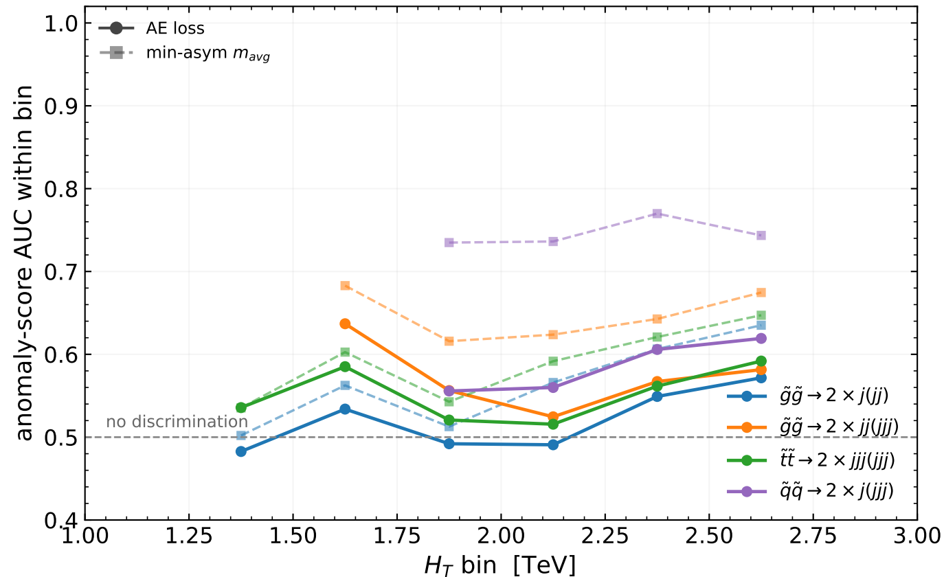
Anomaly-score discrimination at fixed event energy (AUC vs QCD within H_T bins; bins with \geq 30 events per class)
