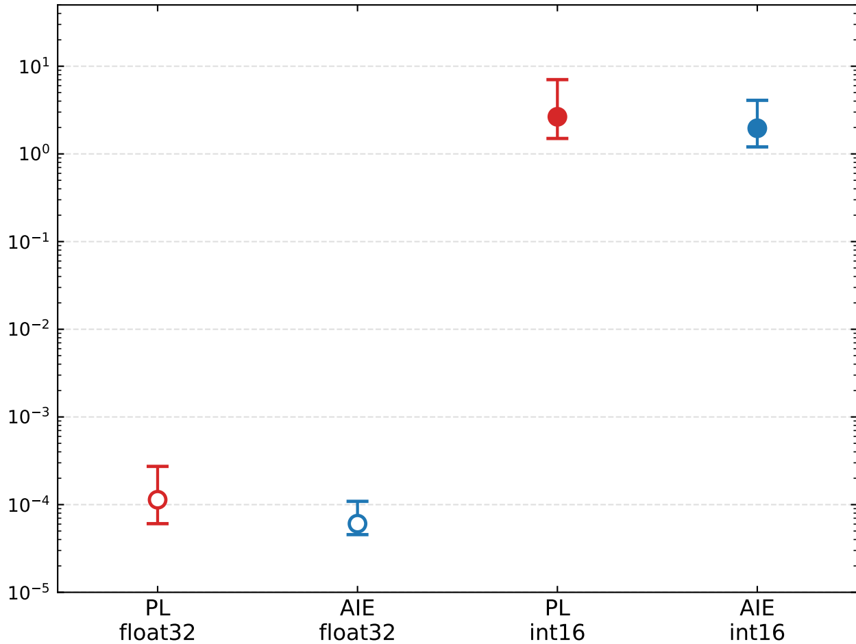
Per-event maximum error vs PyTorch [% of activation RMS]
