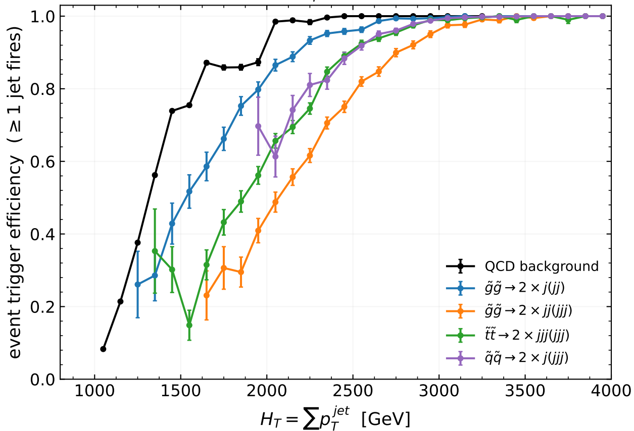
(b) event level — \varepsilon(\geq 1 \text{ jet } p_T^{\text{online}} > T) vs H_T
