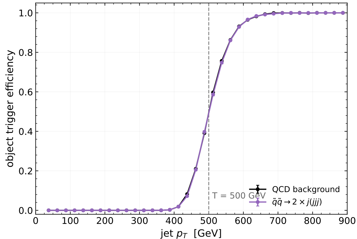
(a) object level — \varepsilon(\text{jet fires}) vs p_T
