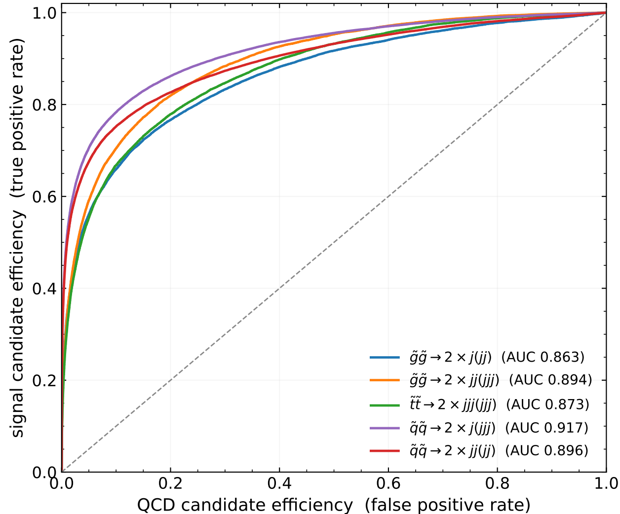
Per-candidate ROC: AE loss of a single BSM candidate (signal vs QCD candidates, retrained model)
