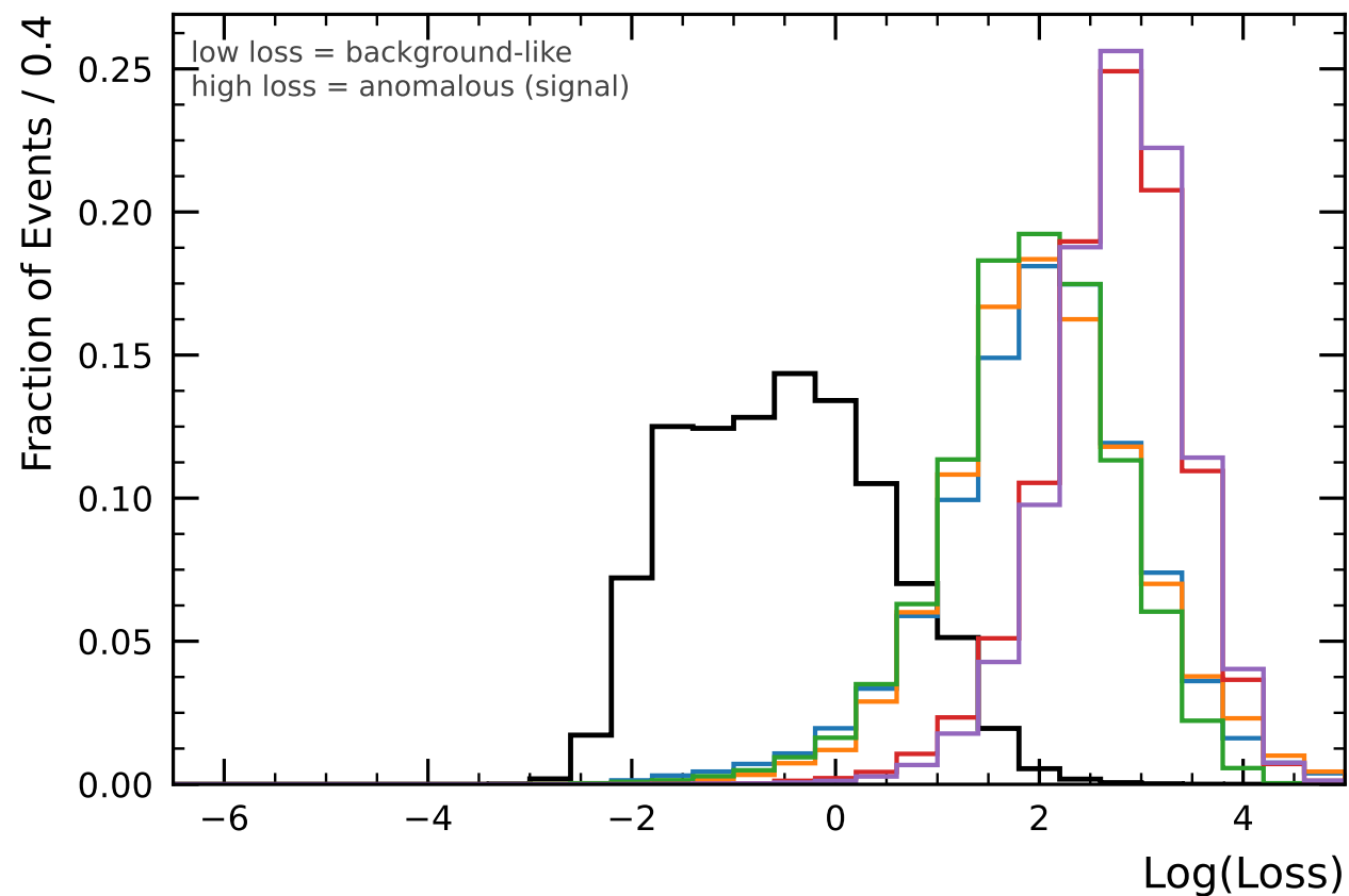
Fig. 2 (bottom) — autoencoder reconstruction loss [new samples + high-stat bkg, seed 5 bestVal]
