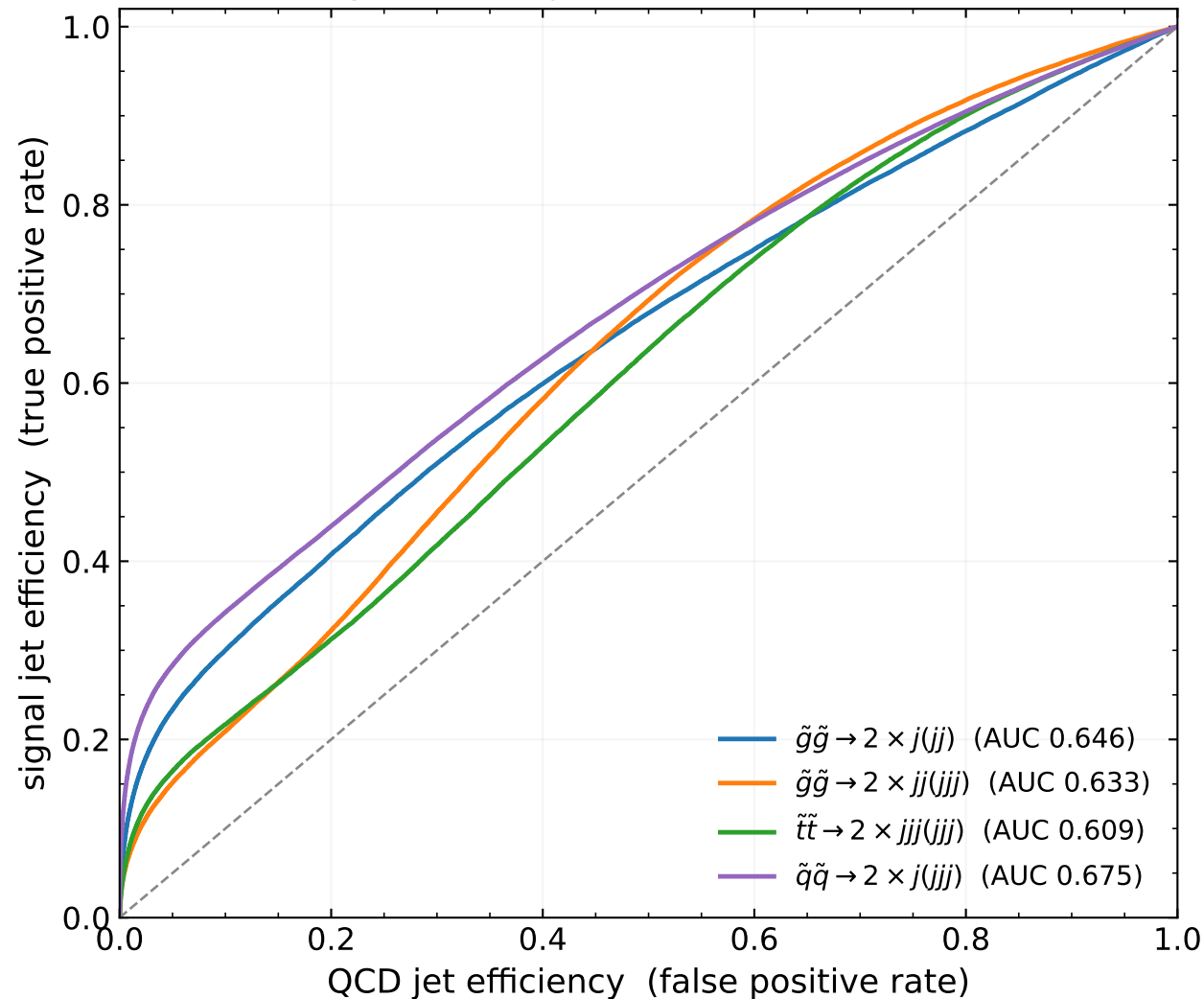
Object-level ROC: online jet p_T as discriminant (signal vs QCD jets, 10% online resolution)
