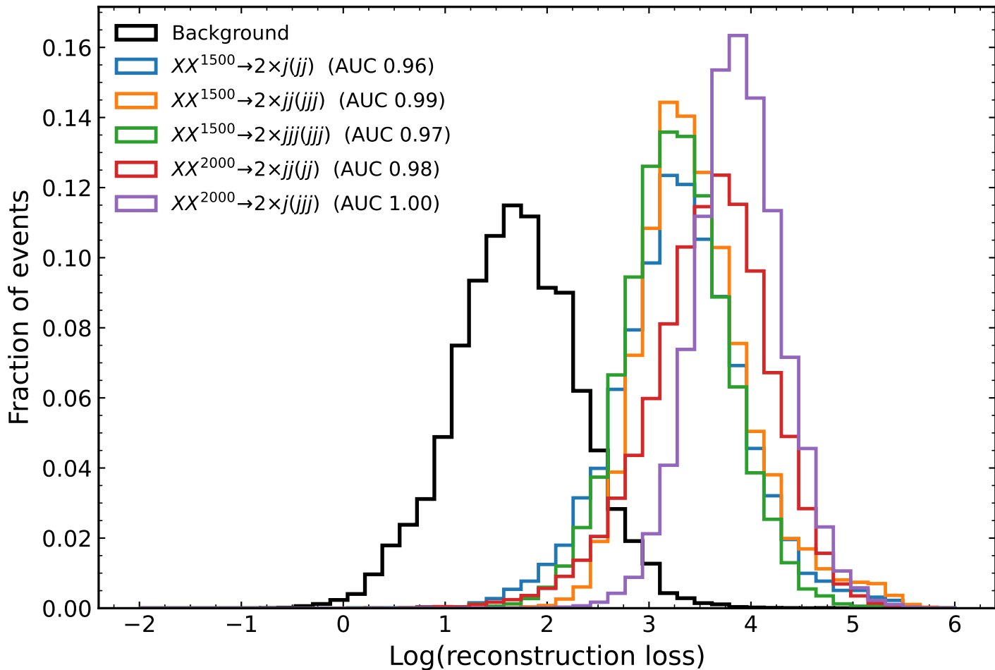
Fig. 2 (bottom) reproduced — retrained non-collapsed model, corrected samples all 5 paper signals separate (AUC 0.96-0.997); background at low loss
