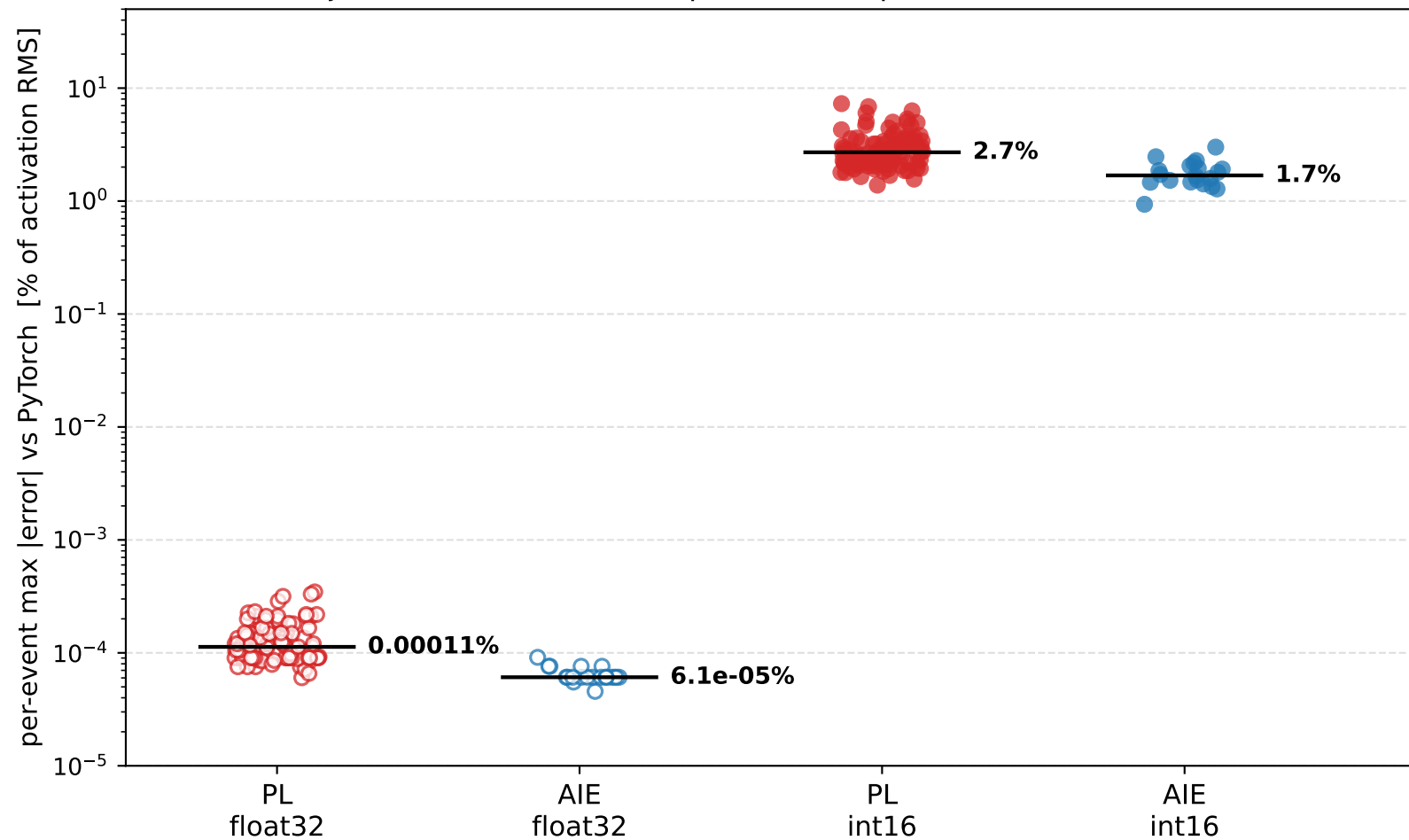
Validation vs PyTorch: same source, two arithmetics (obj self-attention block output; one dot per event; bar = median)
