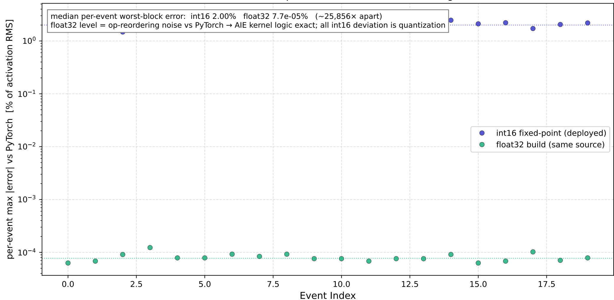
Unquantized Reference: same AIE kernels, two arithmetics, vs PyTorch (worst of the 6 attention blocks per event, x86sim, retrained weights, 20 events)
