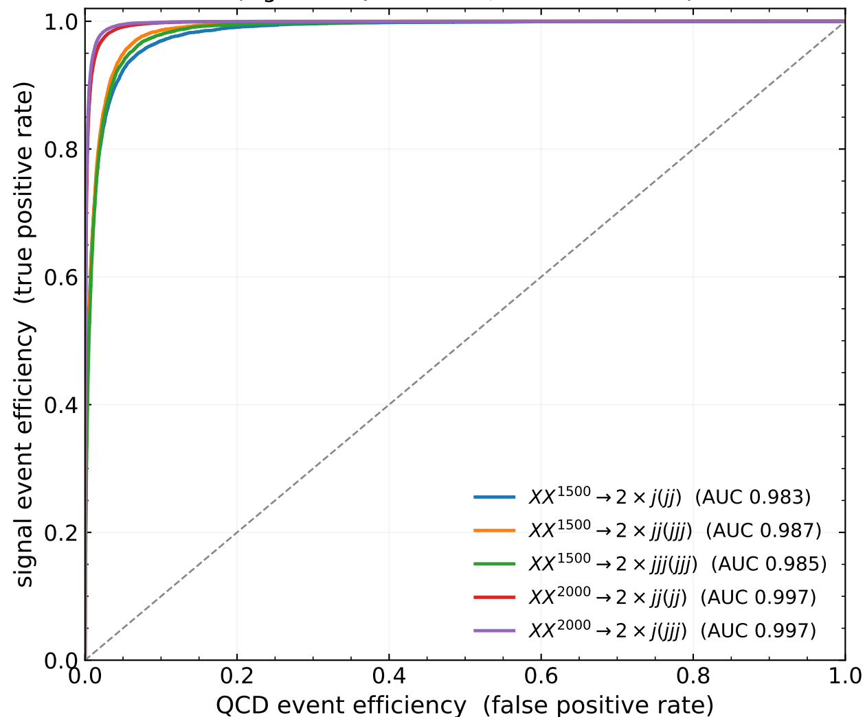
Event-level ROC: AE reconstruction loss as discriminant (signal vs QCD events, retrained model)
