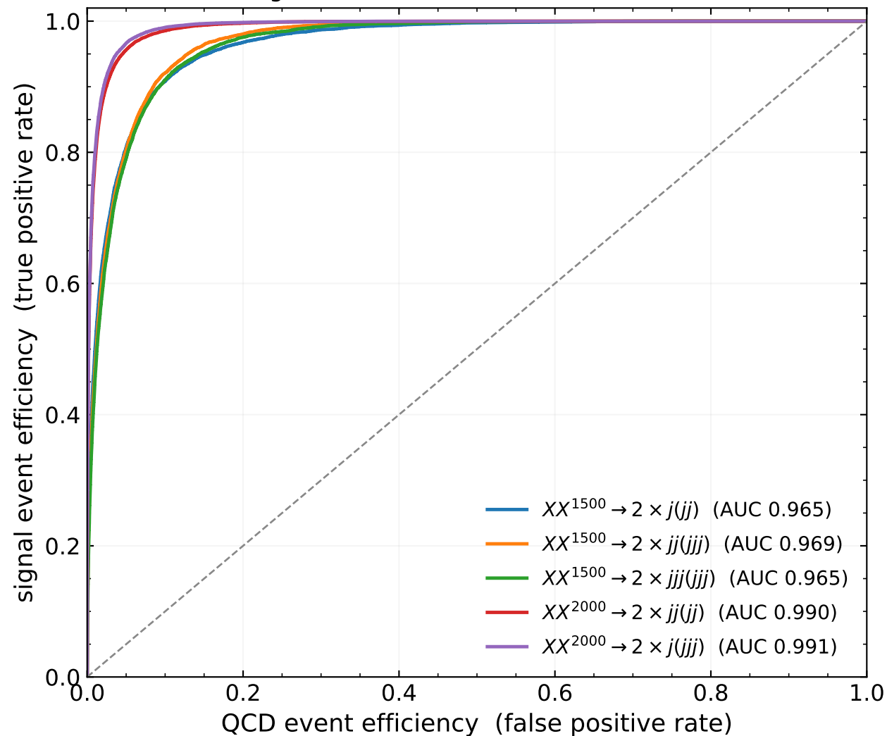
Event ROC: maximum candidate AE loss (signal vs QCD events, retrained model)
