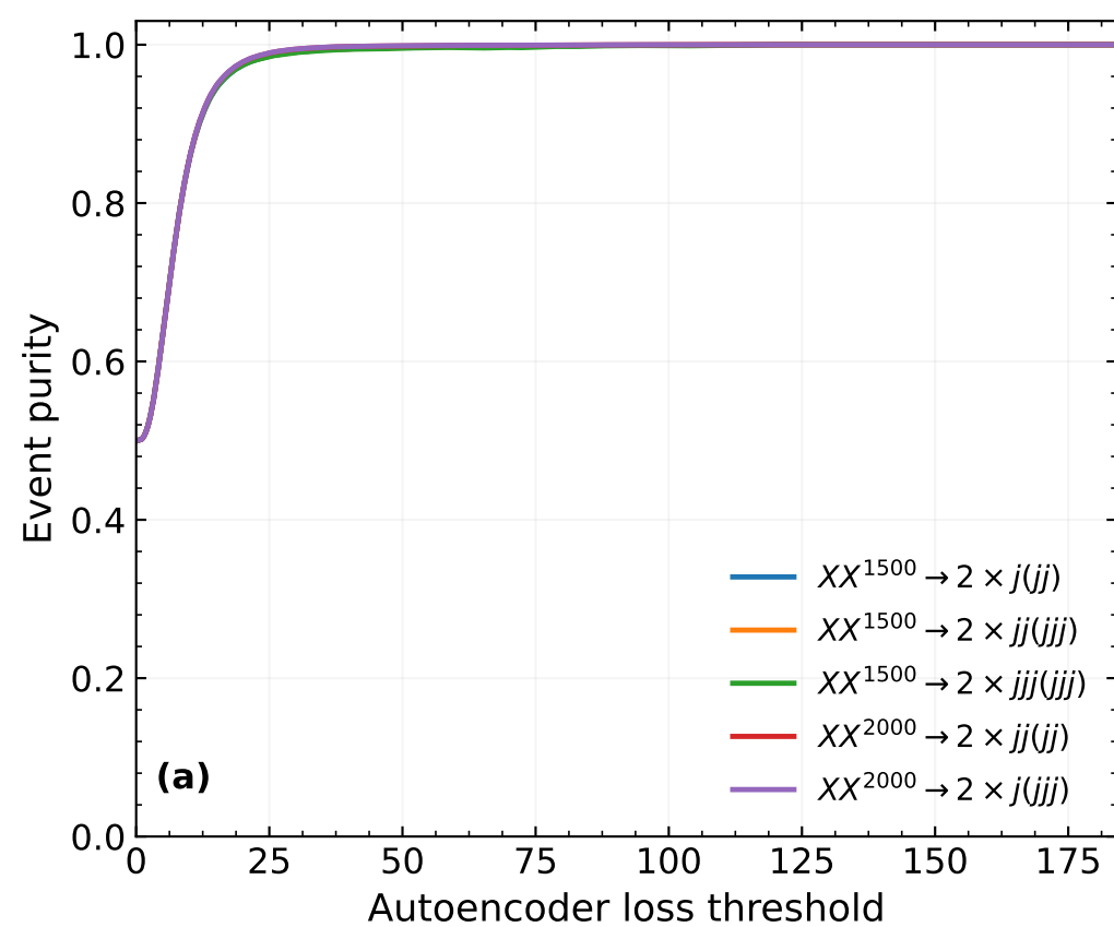
Event-level
