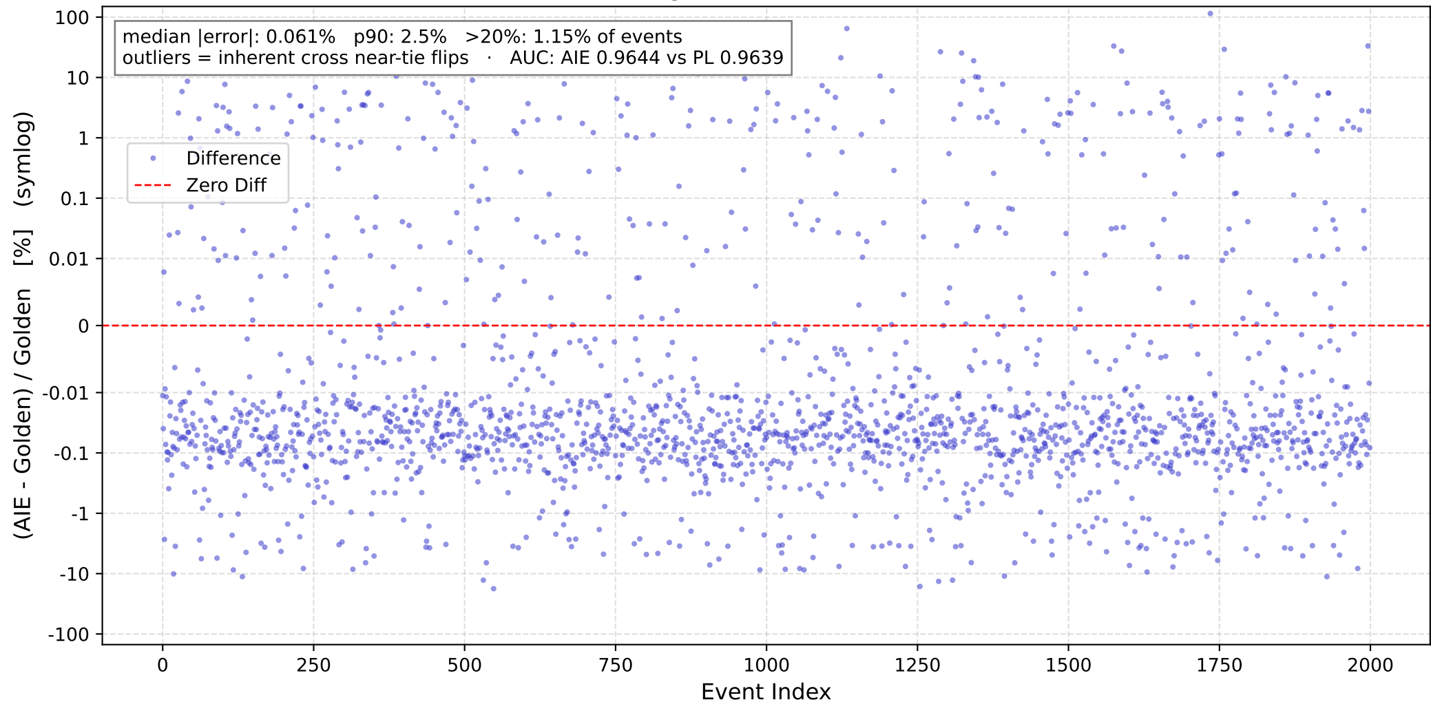
End-to-End Error vs All-PL Golden, per event (final MSE loss, retrained weights, hardware vs hardware, all 2000 events)
