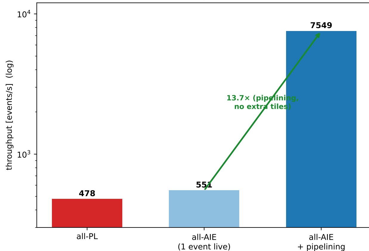
(a) throughput — same 78 tiles, just fed better
