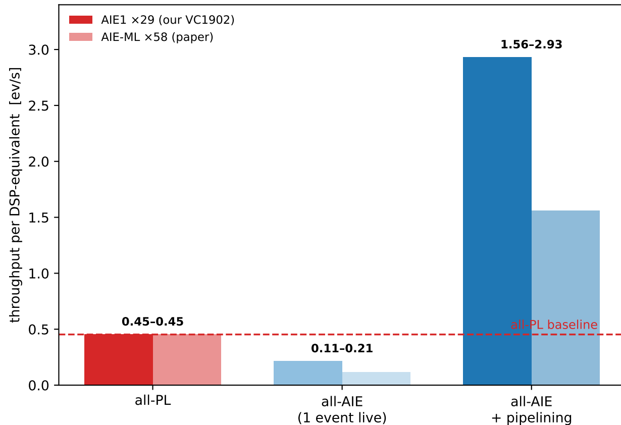
(b) LARE efficiency indicator — pipelining flips the verdict
