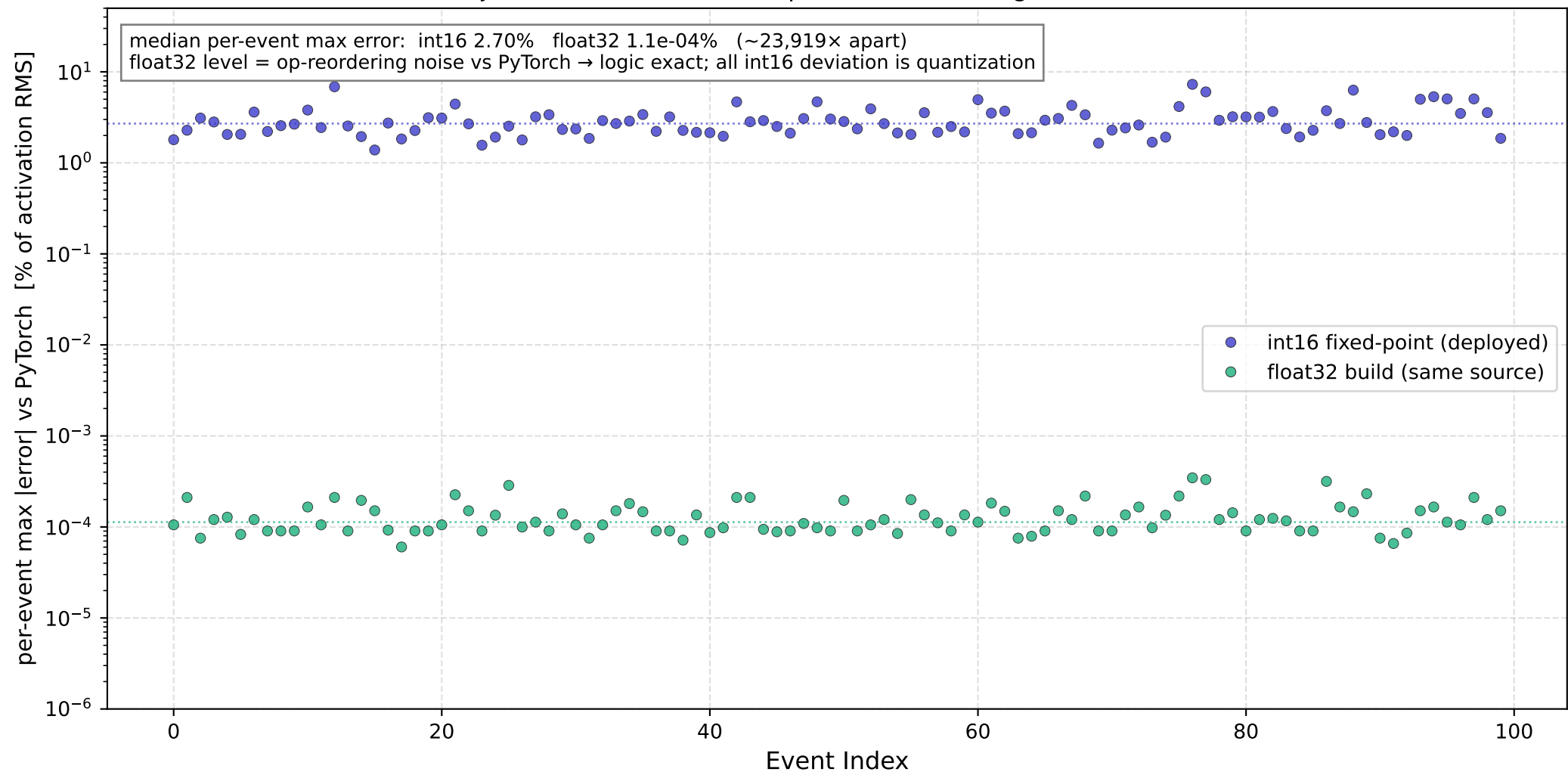
Unquantized Reference: same obj-attention source, two arithmetics, vs PyTorch (obj self-attention block output, retrained weights, 100 events)
