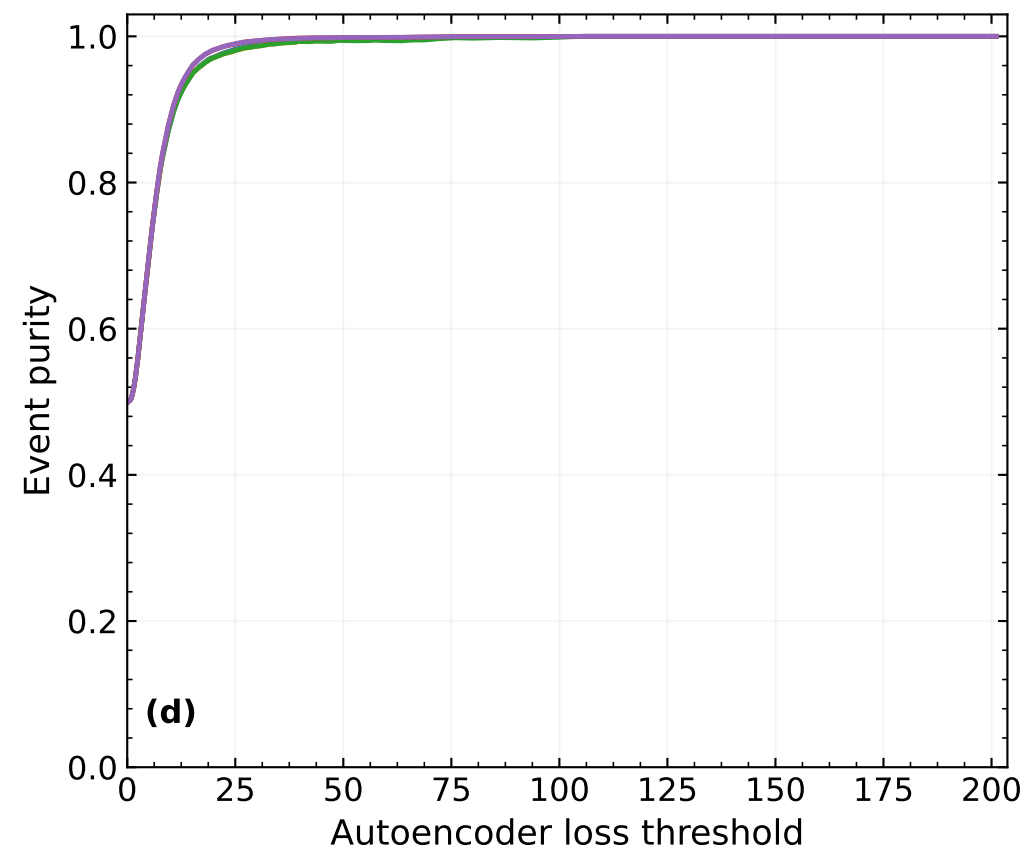
Object-level
