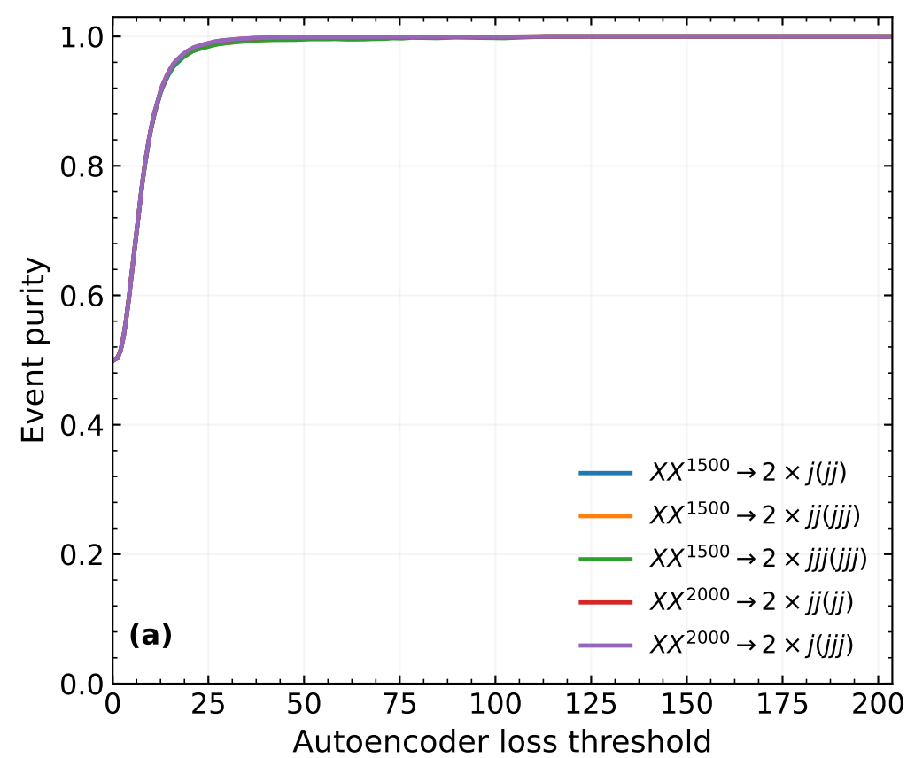
Event-level
