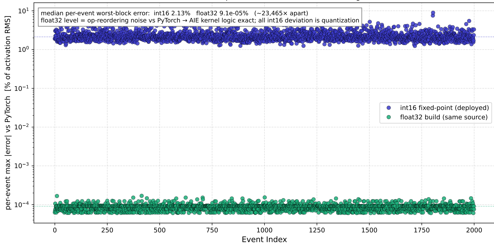
Unquantized Reference: same AIE kernels, two arithmetics, vs PyTorch (worst of the 6 attention blocks per event, x86sim, retrained weights, 2000 events)
