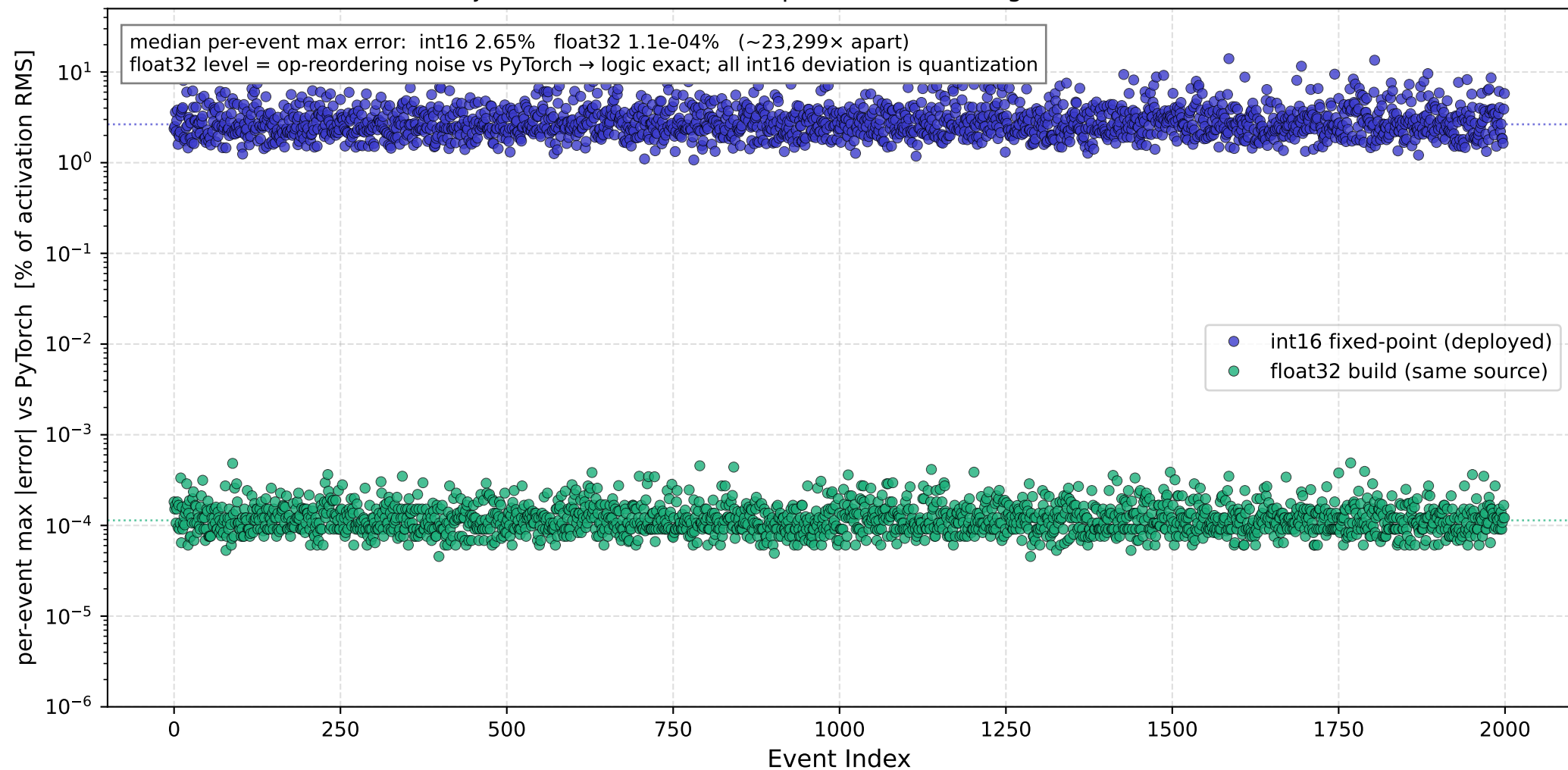
Unquantized Reference: same obj-attention source, two arithmetics, vs PyTorch (obj self-attention block output, retrained weights, 2000 events)
