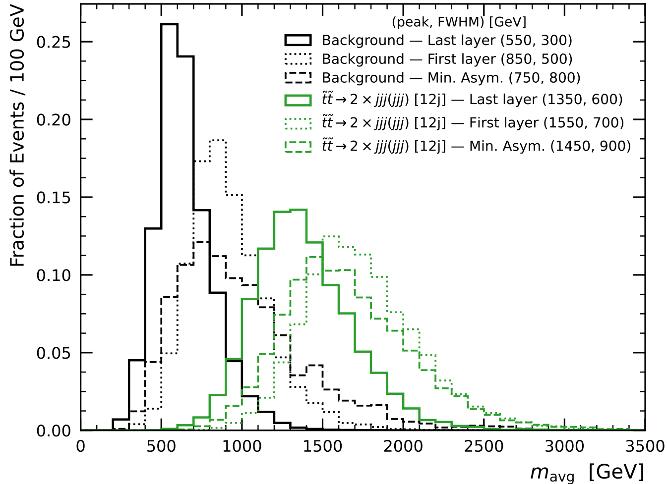
Fig. 3 — last vs first ABC layer vs min-mass-asymmetry
