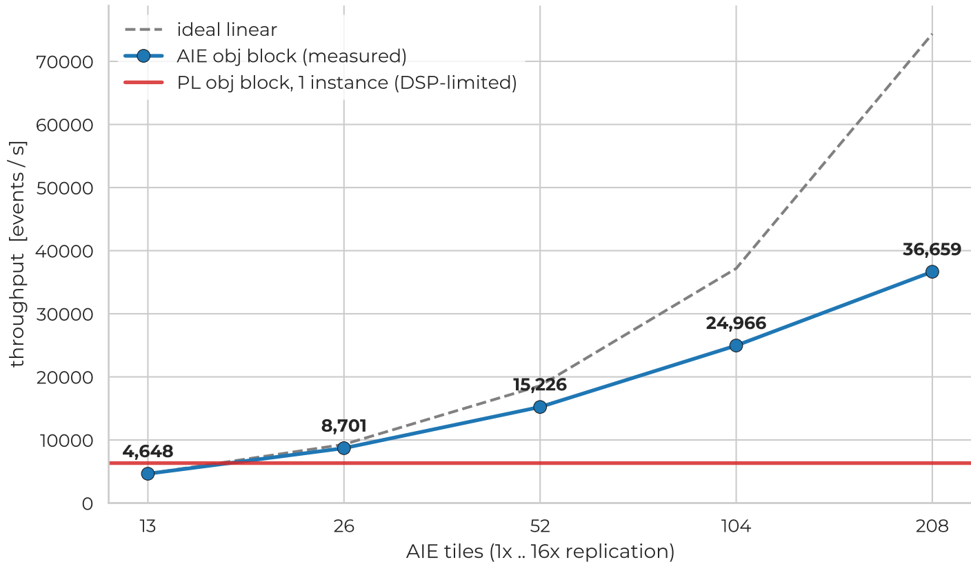
AIE obj-block throughput vs tile replication (measured)
