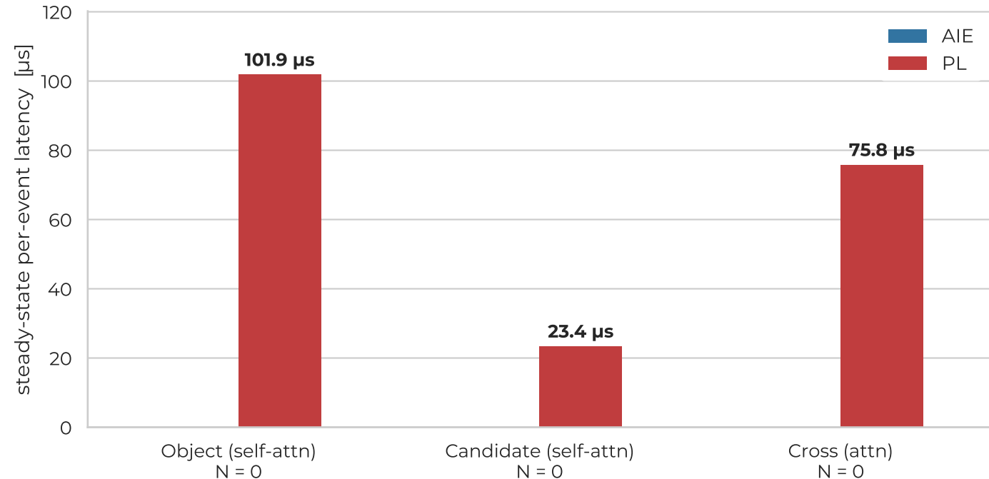
AIE steady-state vs PL per-event latency
