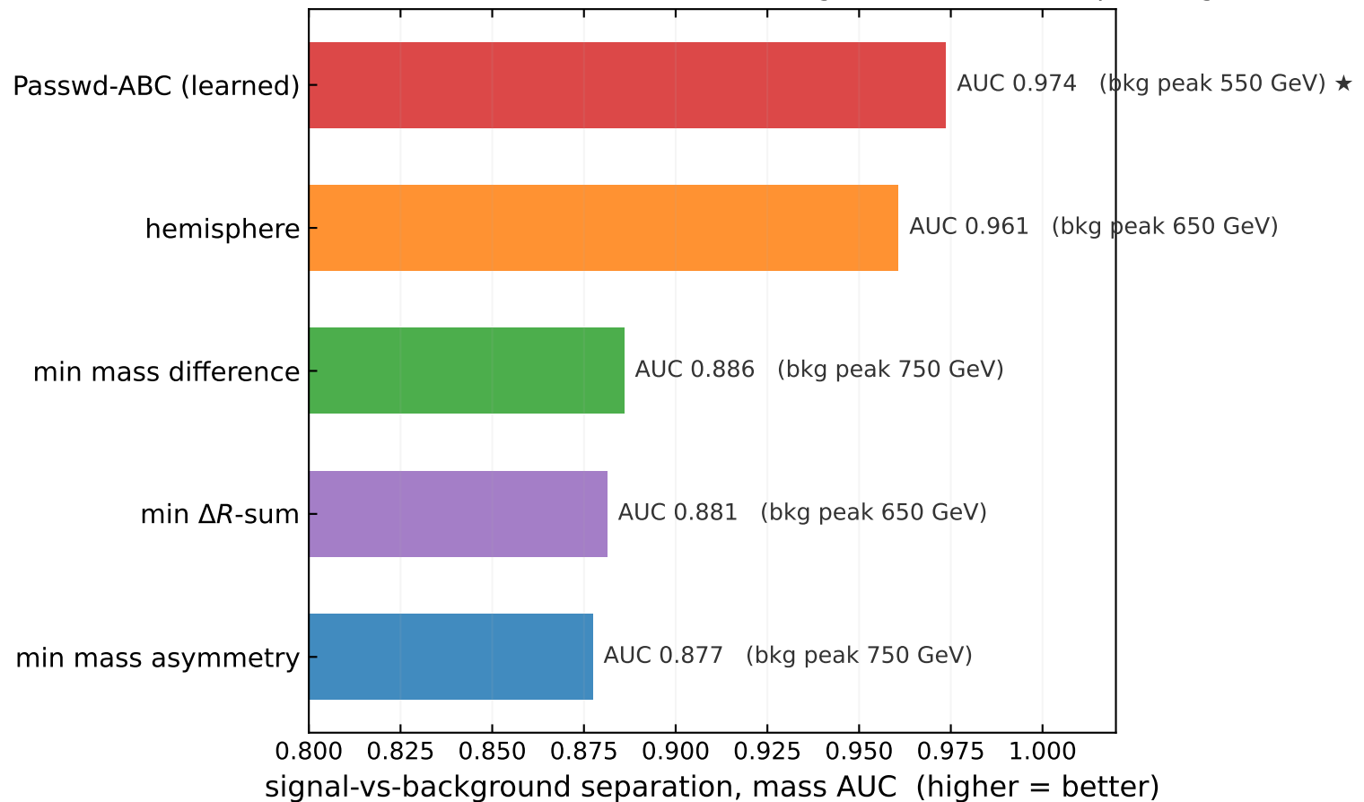
(b) discrimination — the learned assignment doesn't sculpt background
