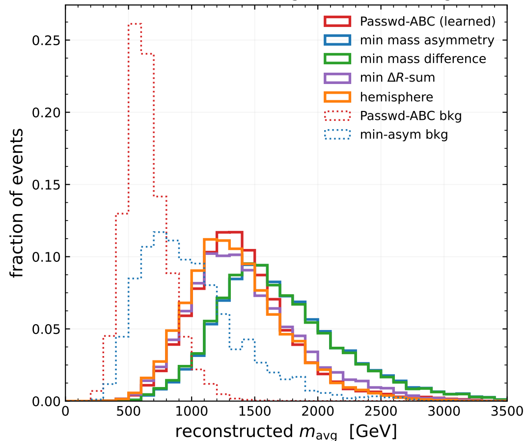
(a) mass reconstruction — signal (solid) vs background (dotted)
