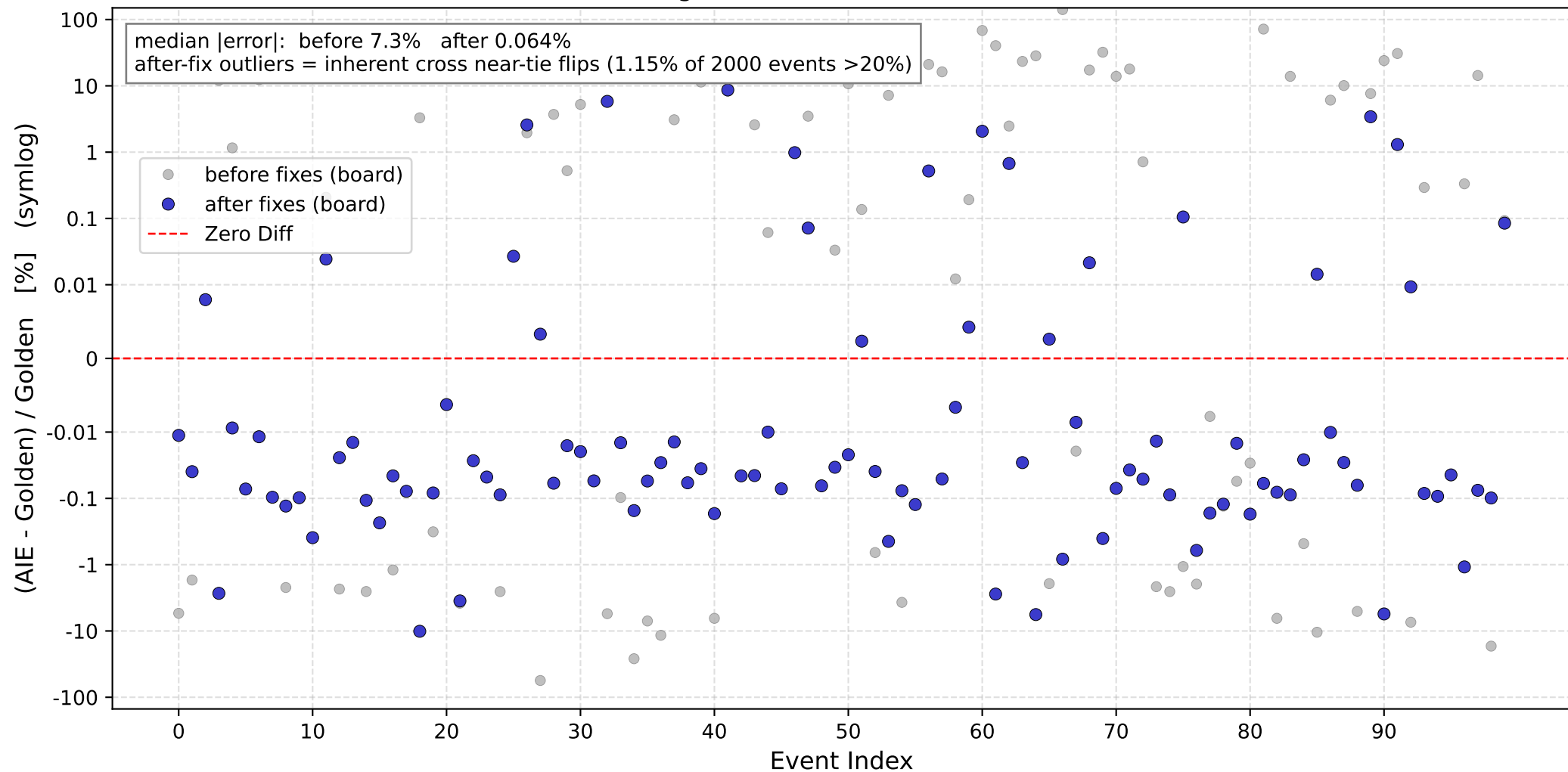
End-to-End Error vs All-PL Golden, per event (final MSE loss, retrained weights, hardware vs hardware, first 100 of 2000 events)
