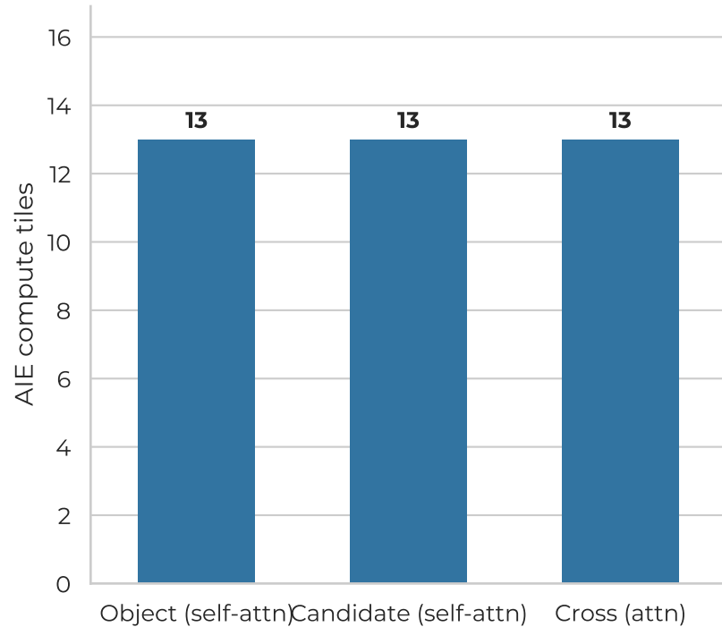
AIE tile usage (39/400 = 9.8% of array)
